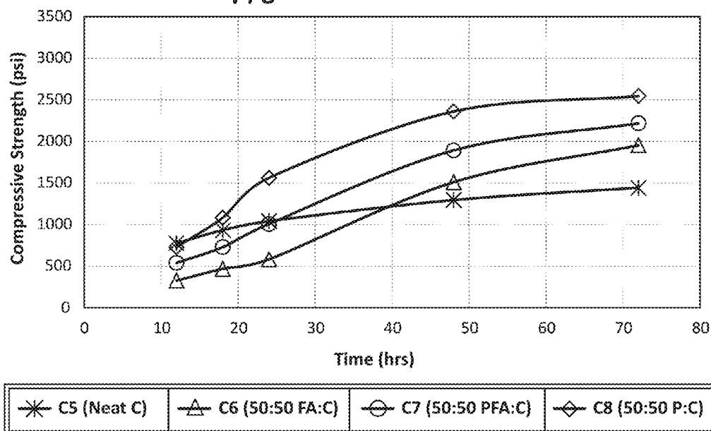
Compressive Strength Over Time Set 3: 14.2 ppg Class C Cement Slurries
