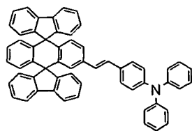
Chemical Compound 400
