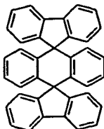
Chemical Compound 12
