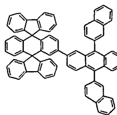
Chemical Compound 117
