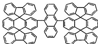
Chemical Compound 102
