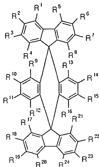
Chemical Formula 1
