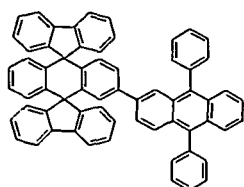
Chemical Compound 116
