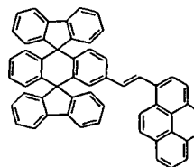
Chemical Compound 103
