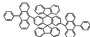
Chemical Compound 114
