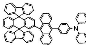
Chemical Compound 401
