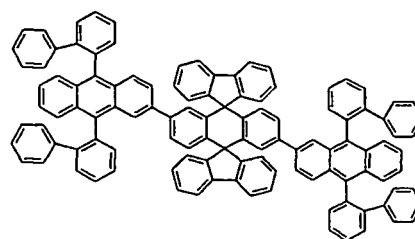
Chemical Compound 121
