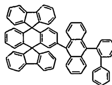
Chemical Compound 111
