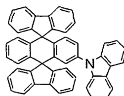
Chemical Compound 10
