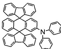
Chemical Compound 11
