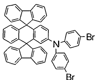
Chemical Compound 7
