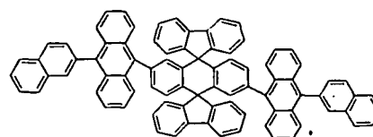
Chemical Compound 115
