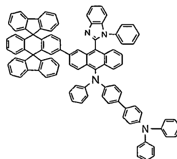
Chemical Compound 125
