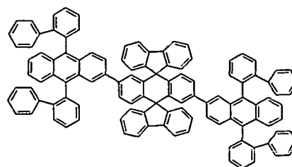
Chemical Compound 121
