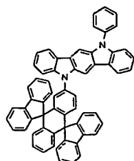
Chemical Compound 410
