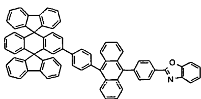
Chemical Compound 126
