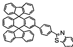
Chemical Compound 213
