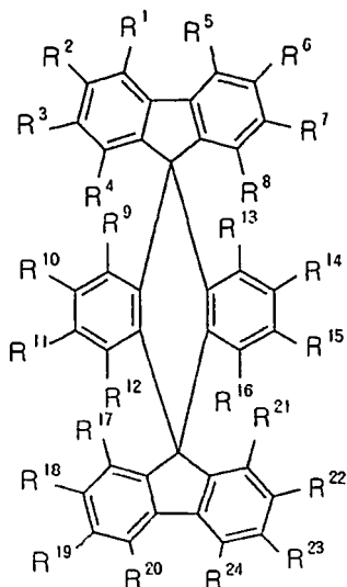
General Formula 1
