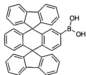
Chemical Compound 8
