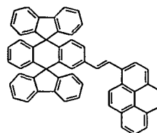
Chemical Compound 103
