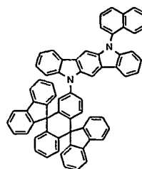
Chemical Compound 411
