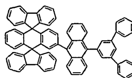
Chemical Compound 113
