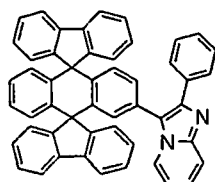
Chemical compound 412
