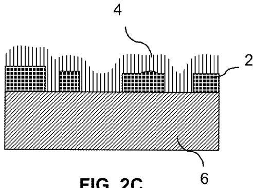
FIG. 2C (PRIOR ART)
