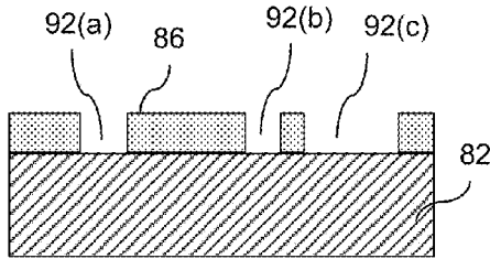
FIG. 4C (PRIOR ART)
