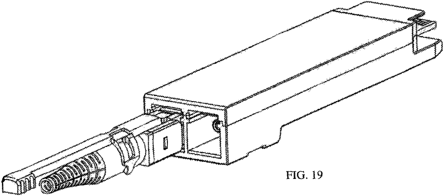
QSFP WITH ONE DUAL FERRULE CONNECTOR INSERTED
