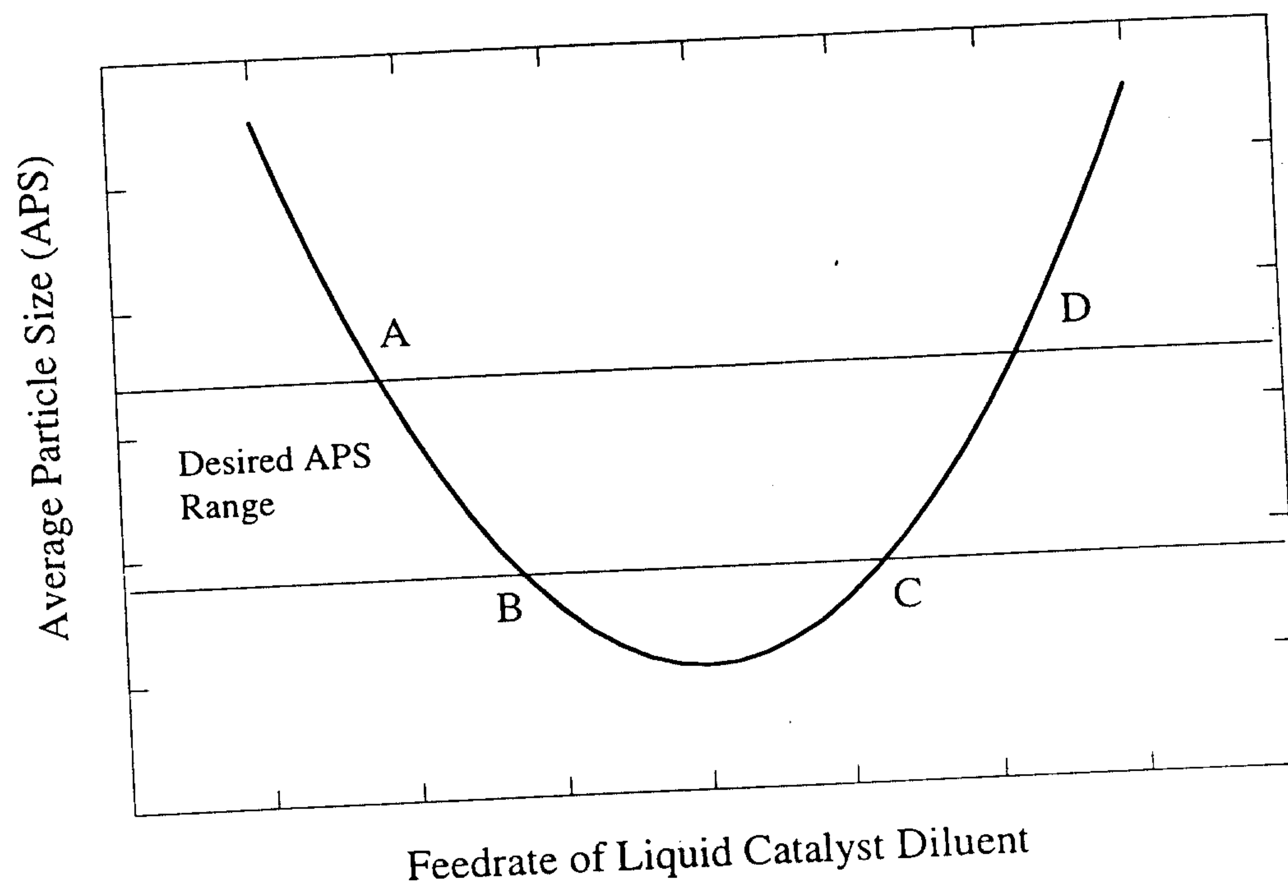
Figure 4. Effect of liquid catalyst diluent addition on particle size.
