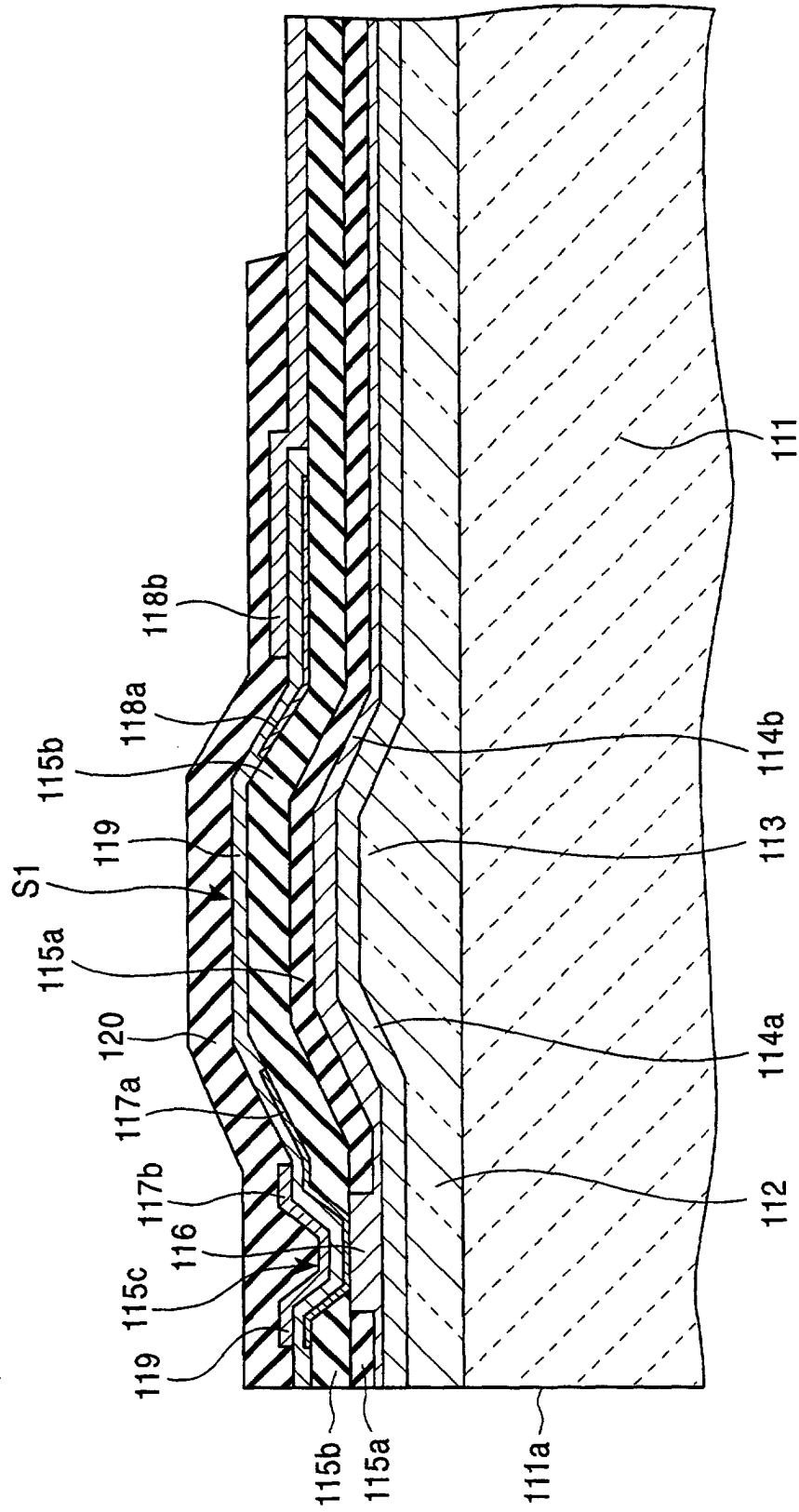
FIG. 15 PRIOR ART
