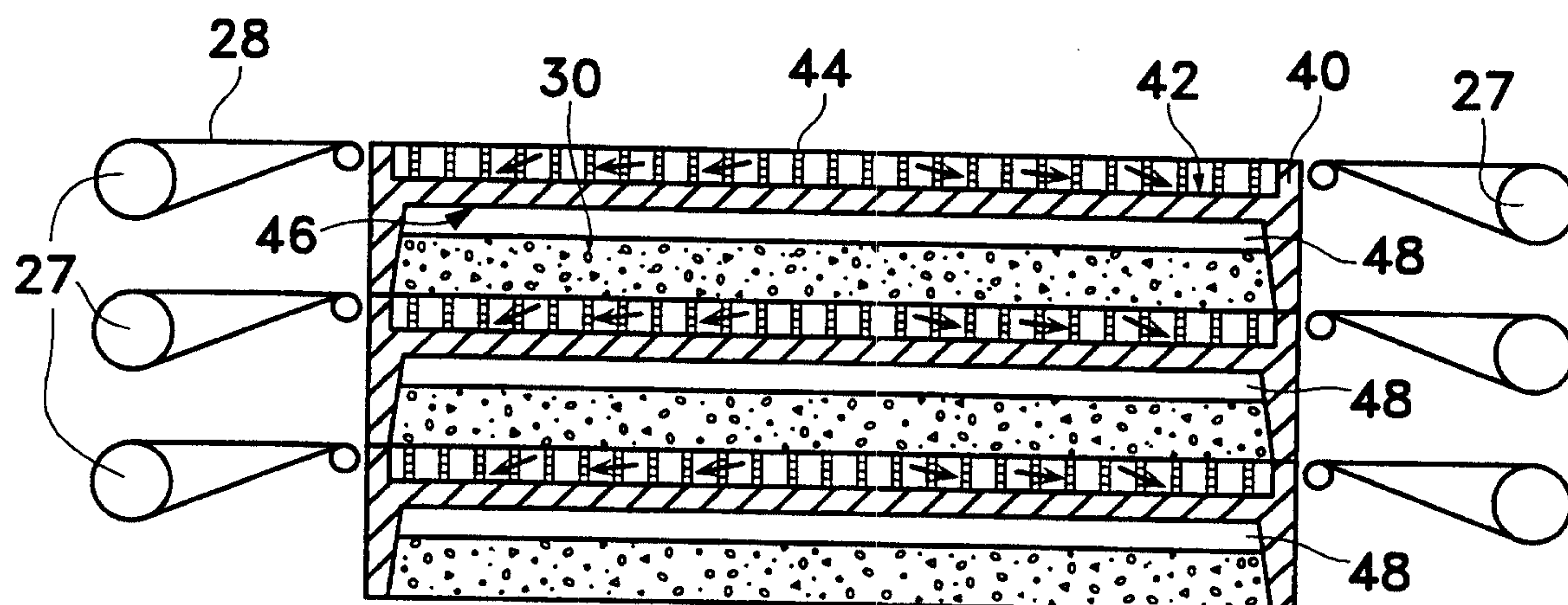
FIG. 7 PLATES CLOSED
