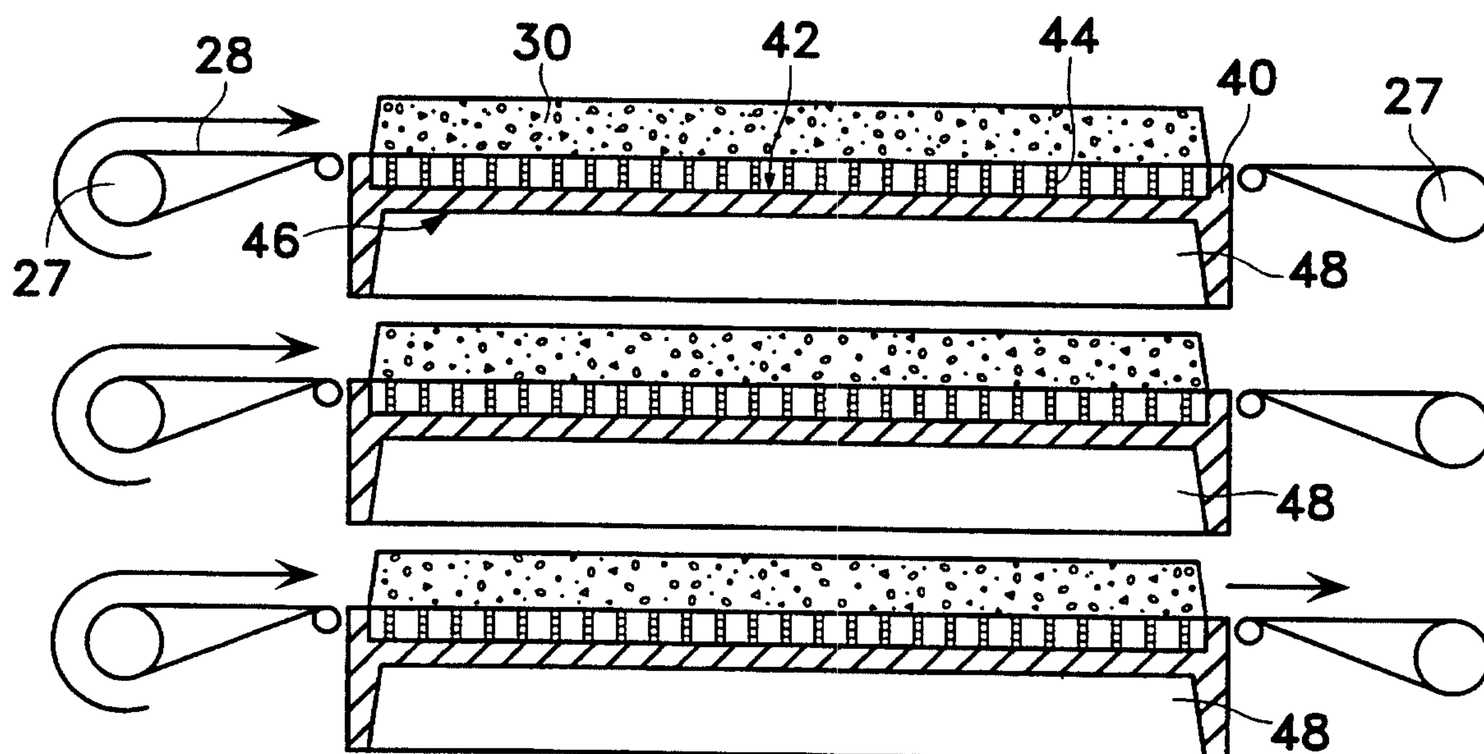
FIG. 8 PLATES OPEN
