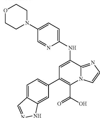
6-(1H-indazol-6-yl)-8-(5-morpholinopyridin-2-ylamino)imidazo[1,2-a]pyridine-5-carboxylic acid
