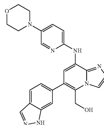
(6-(1H-indazol-6-yl)-8-(5-morpholinopyridin-2-ylamino)imidazo[1,2-a]pyridin-5-yl)methanol 9
