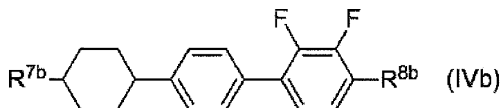
[Chem. 12]
