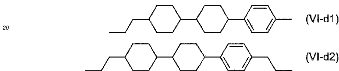
[Chem. 22]
