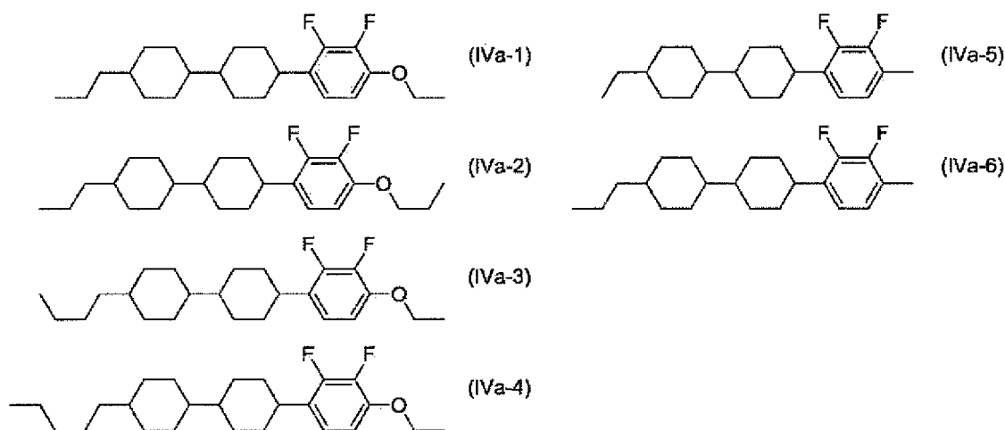
[Chem. 11]
