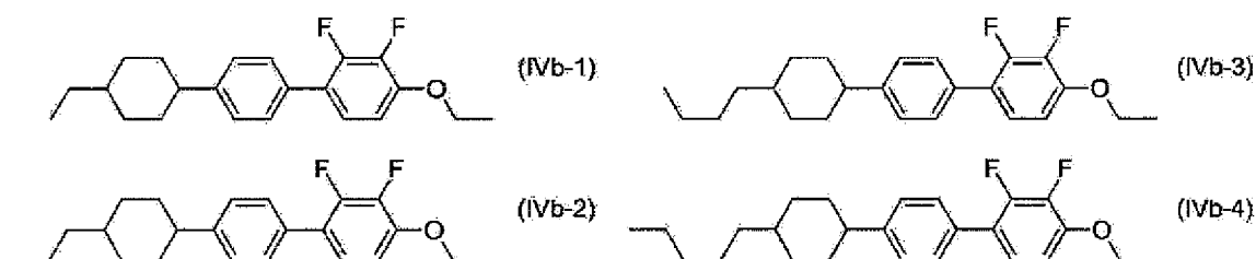
[Chem. 13]
