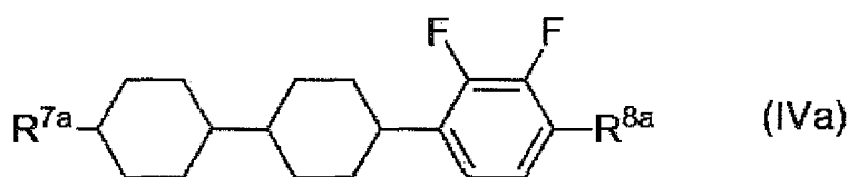
[Chem. 10]
