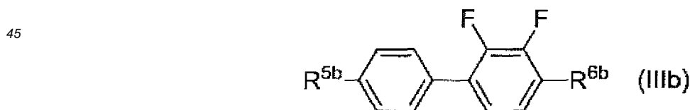
[Chem. 7]
