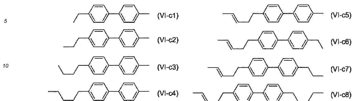
[Chem. 21]
