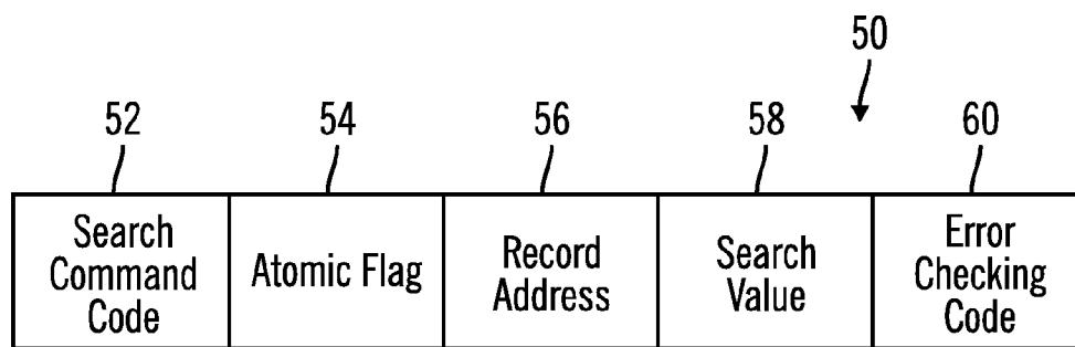
Search Command
