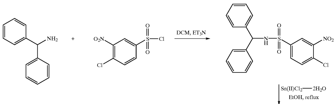
Scheme X
