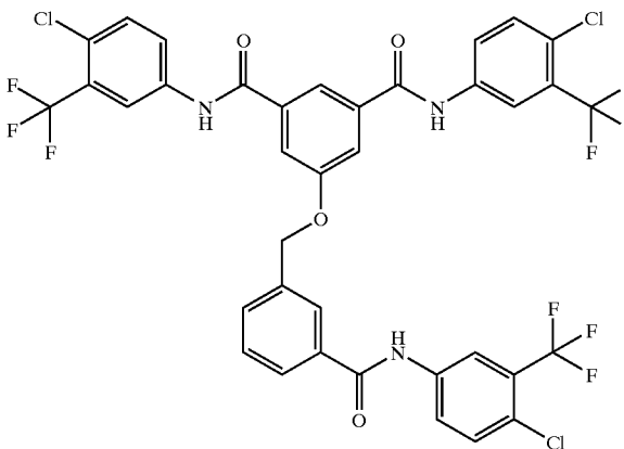
Compound # 37
