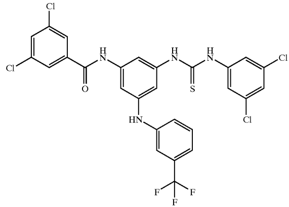
Compound # 10
