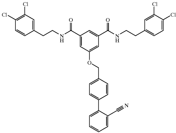
Compound # 21
