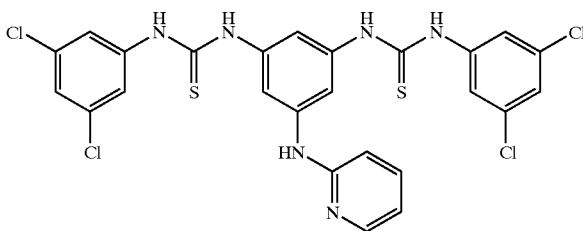
Compound # 13
