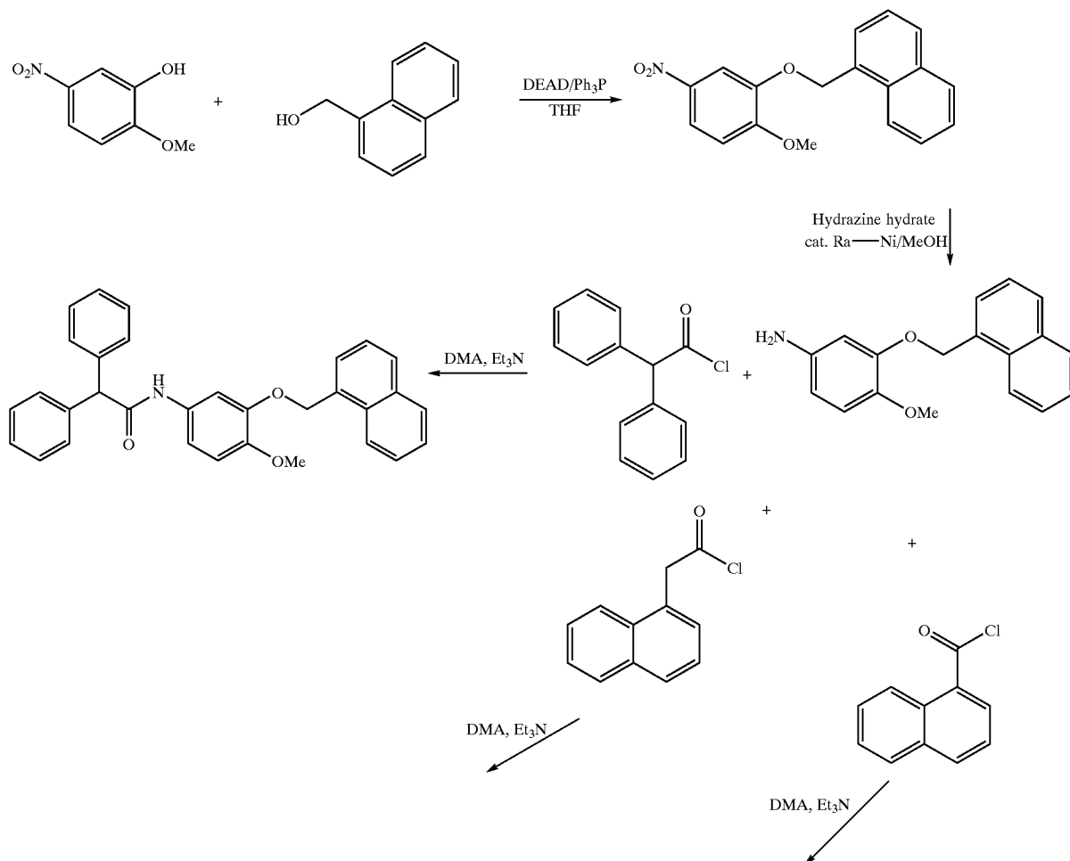
Scheme XIII
