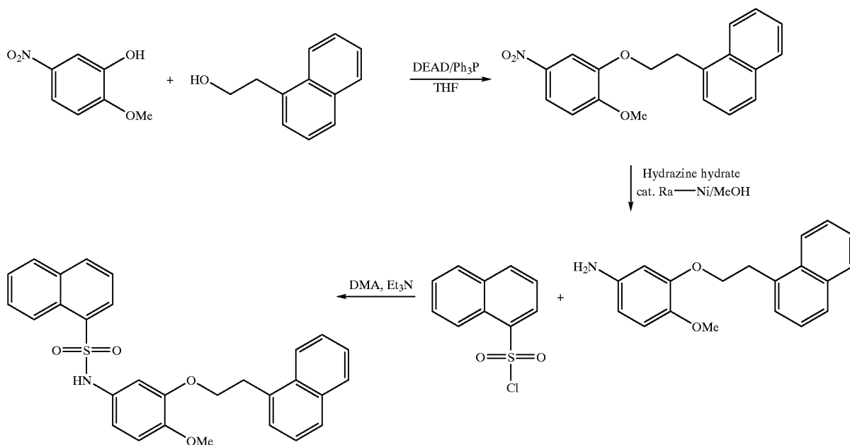
Scheme XII
