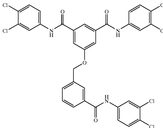
Compound # 38
