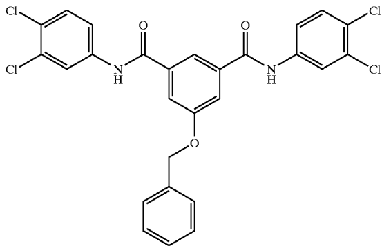
Compound # 43
