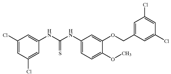
Compound # 28
