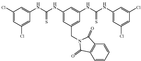
Compound # 27
