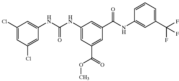
Compound # 5
