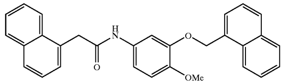
Compound # 48
