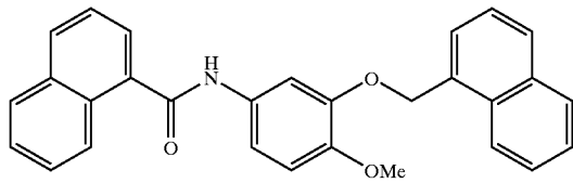
Compound # 47
