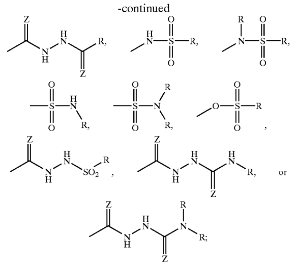
Formula I
