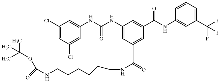
Compound # 5
