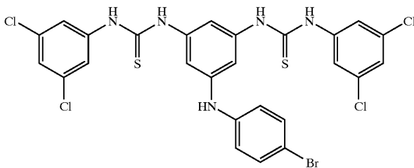
Compound # 11
