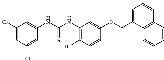
Compound # 35
