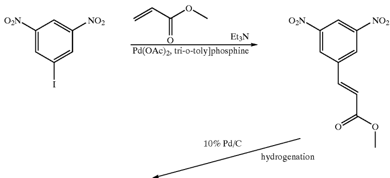
Scheme III-A
