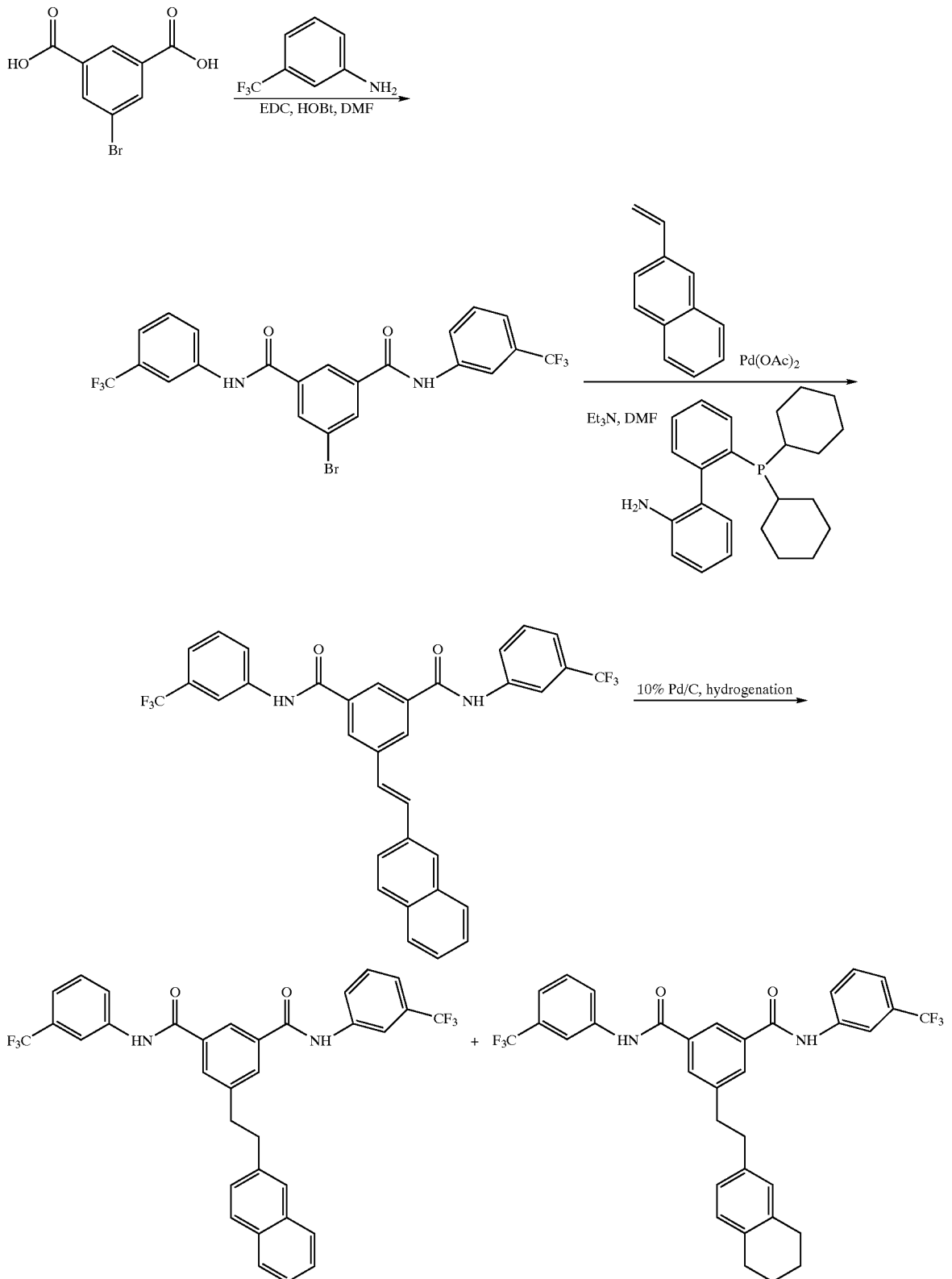
Scheme I-F
