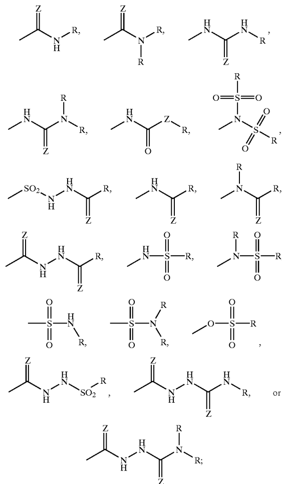
Formula I
