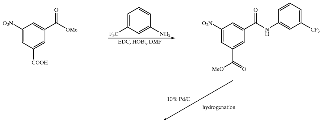
Scheme III-B
