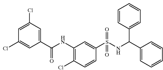
Compound # 52
