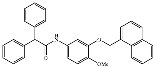
Compound # 49
