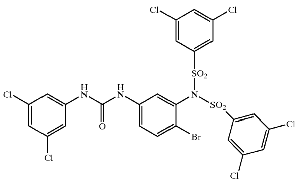
Compound # 29
