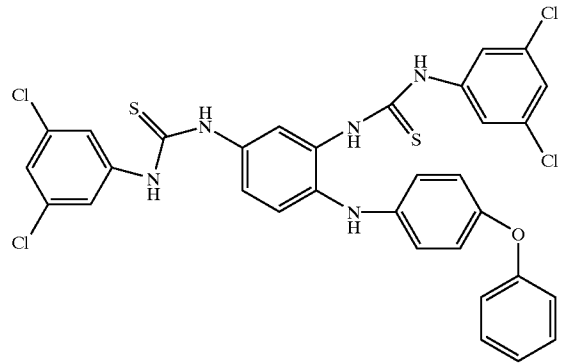
Compound # 40
