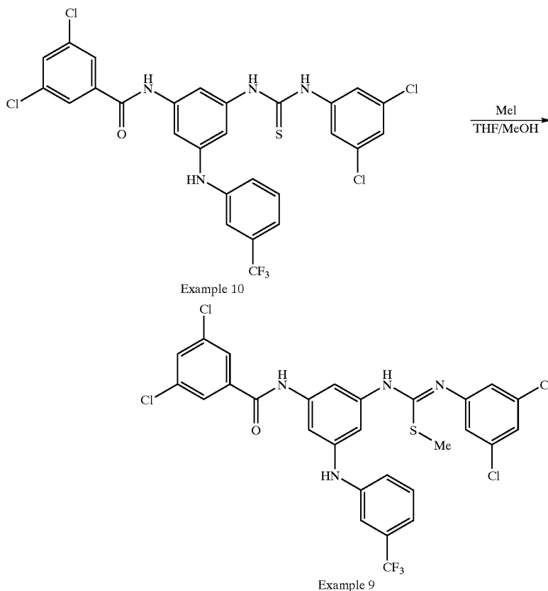
Scheme II-C
