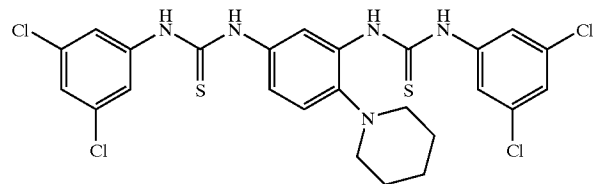
Compound # 44
