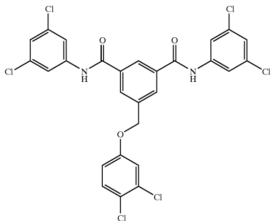
Compound # 20
