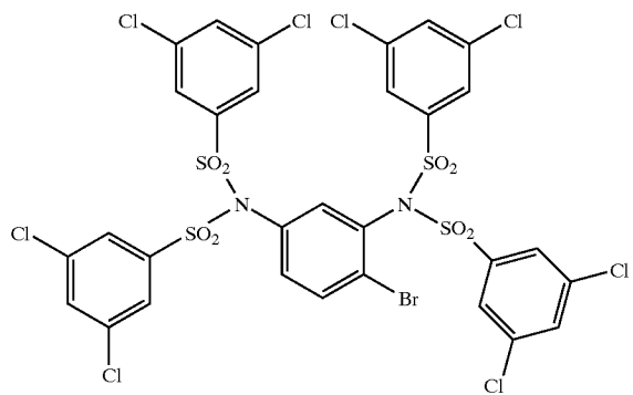
Compound # 30
