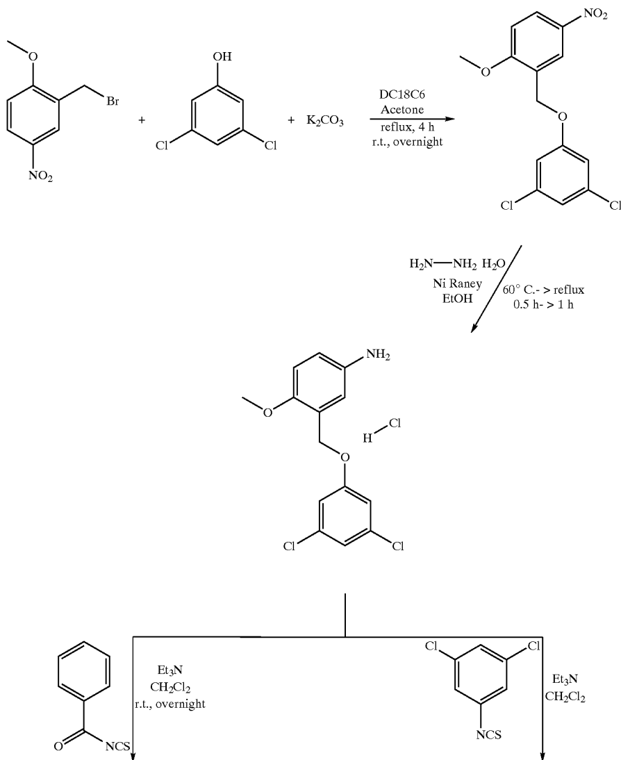
Scheme VIII
