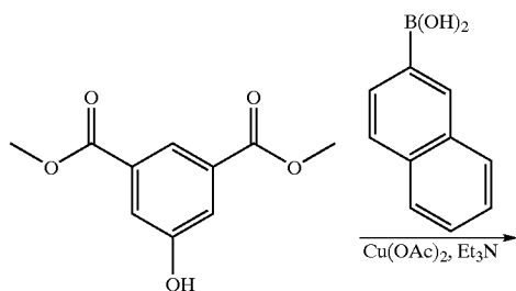
Scheme I-D
