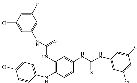
Compound # 38
