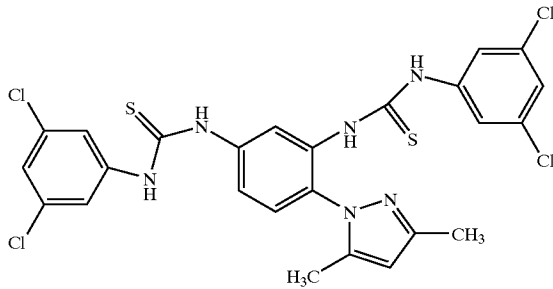
Compound # 39
