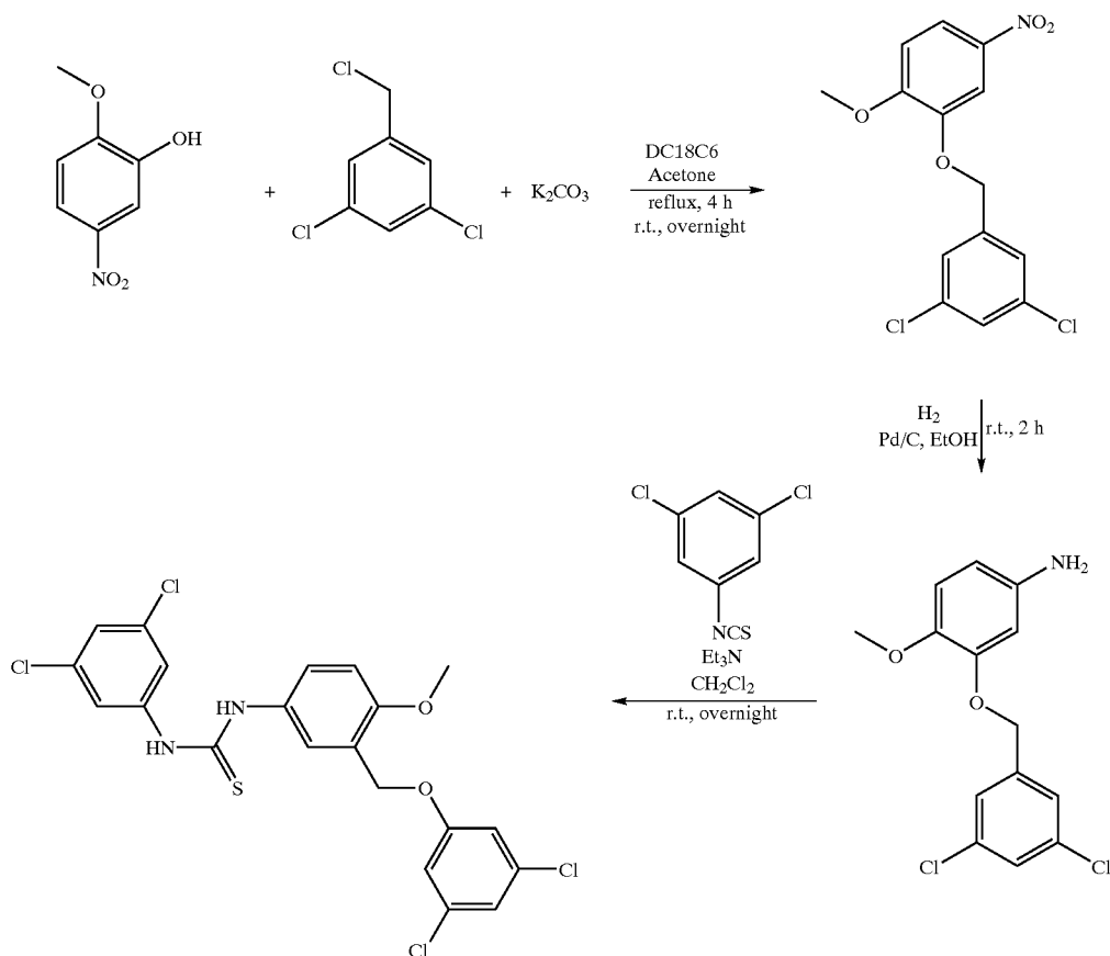
Scheme IX
