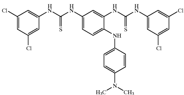
Compound # 35
