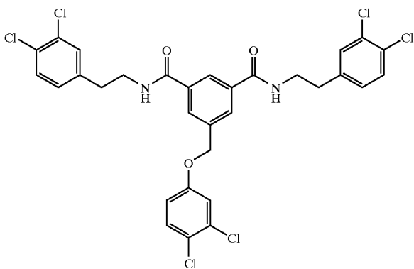
Compound # 19
