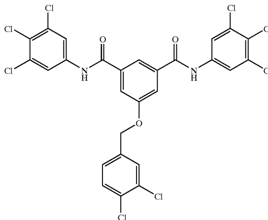
Compound # 34
