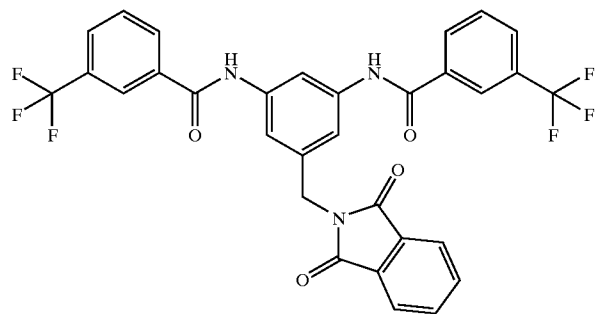
Compound # 12
