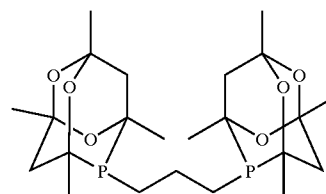
1,3-P,P'-di(2-phospha-1,3,5,7-tetramethyl-6,9,10-trioxatricyclo[3.3.1.1{3.7}]decylpropane ("dpa-3").
