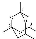
1,3,5,7-tetramethyl-4,8,9-trioxa-3,7-bicyclo[3.3.1]nonylene.
