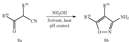
Scheme 8:
