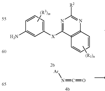
Scheme 4:
