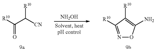
Scheme 9:
