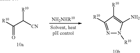
Scheme 10:
