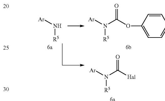
Scheme 6:
