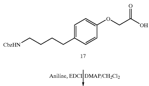
Scheme 4. Synthesis of PSA 17482
