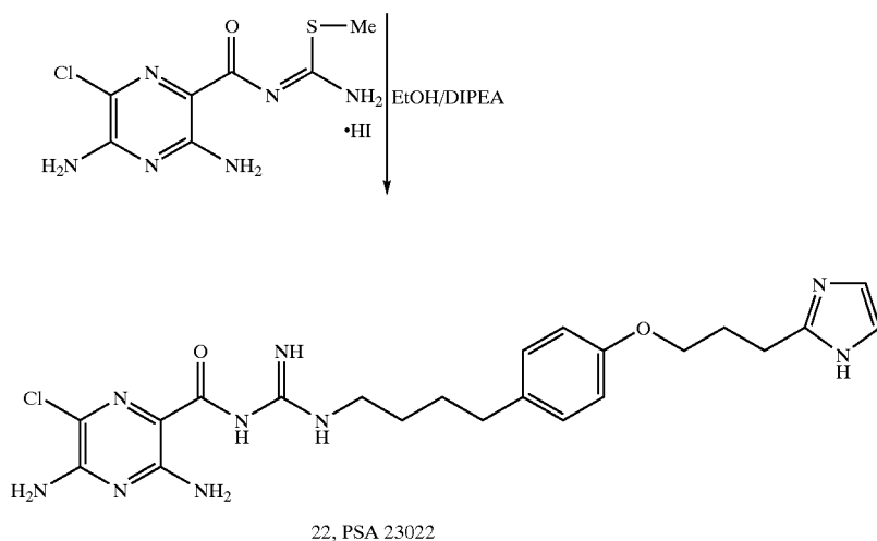
Scheme 6. Synthesis of PSA 16826
