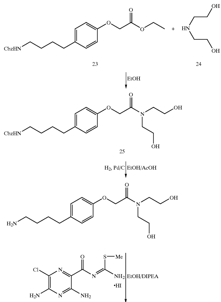
Scheme 6. Synthesis of PSA 16826
