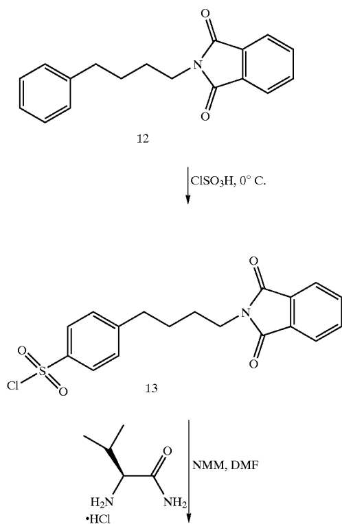
Scheme 3. Synthese of PSA 19008
