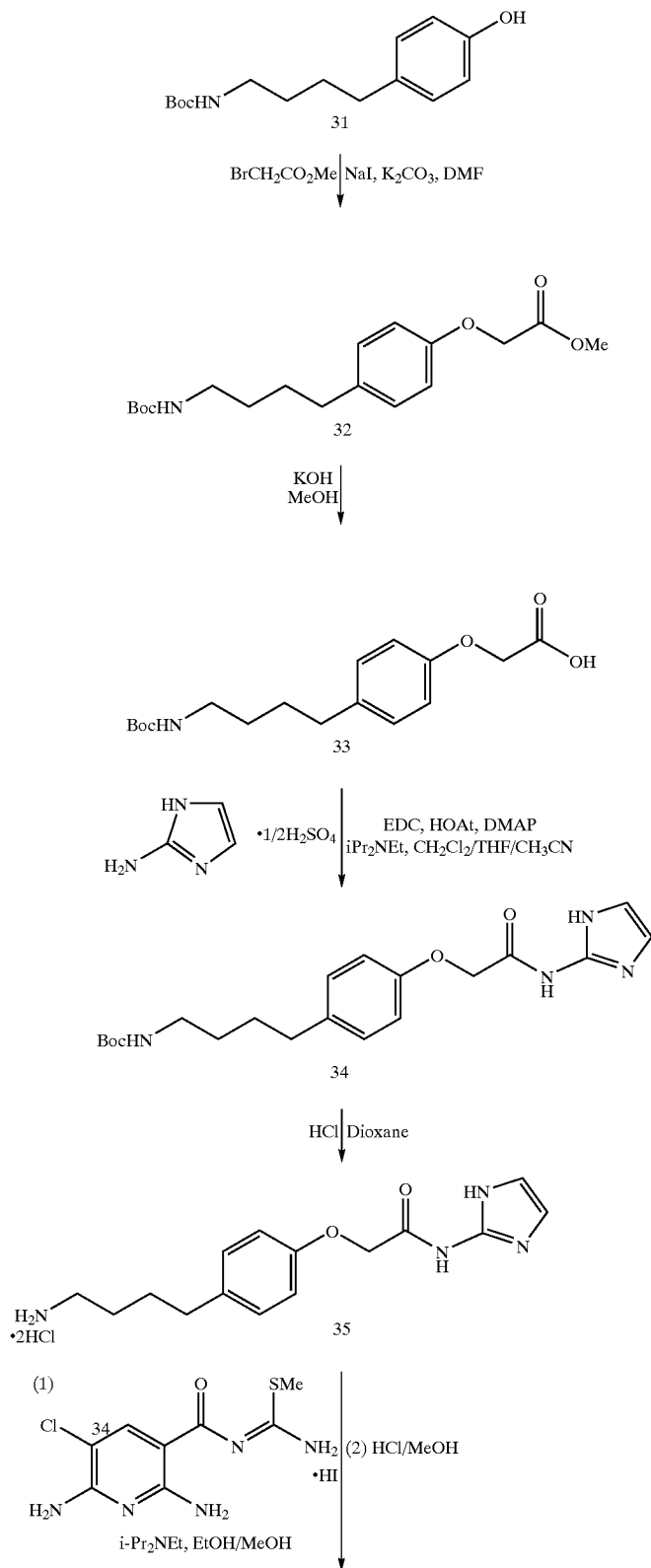
Scheme 8. Synthesis of PSA 16437
