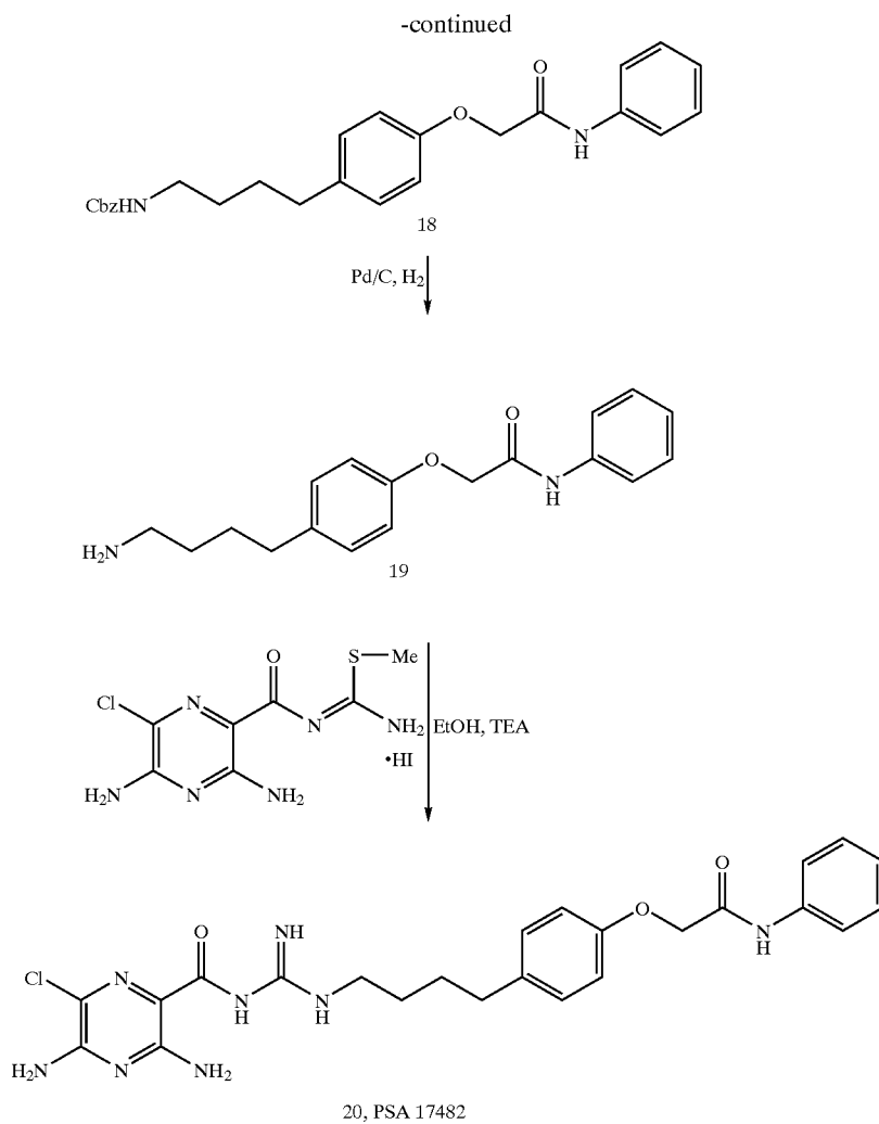
Scheme 5. Synthesis of PSA 23022
