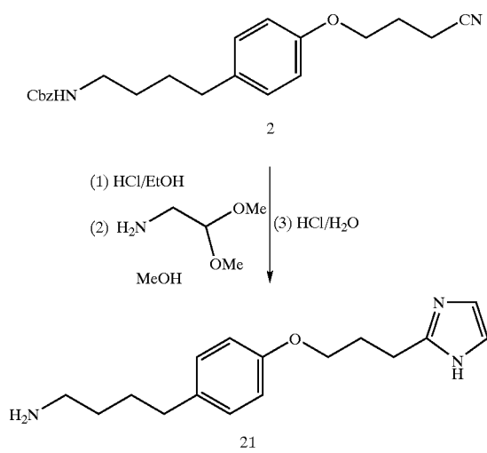
Scheme 5. Synthesis of PSA 23022
