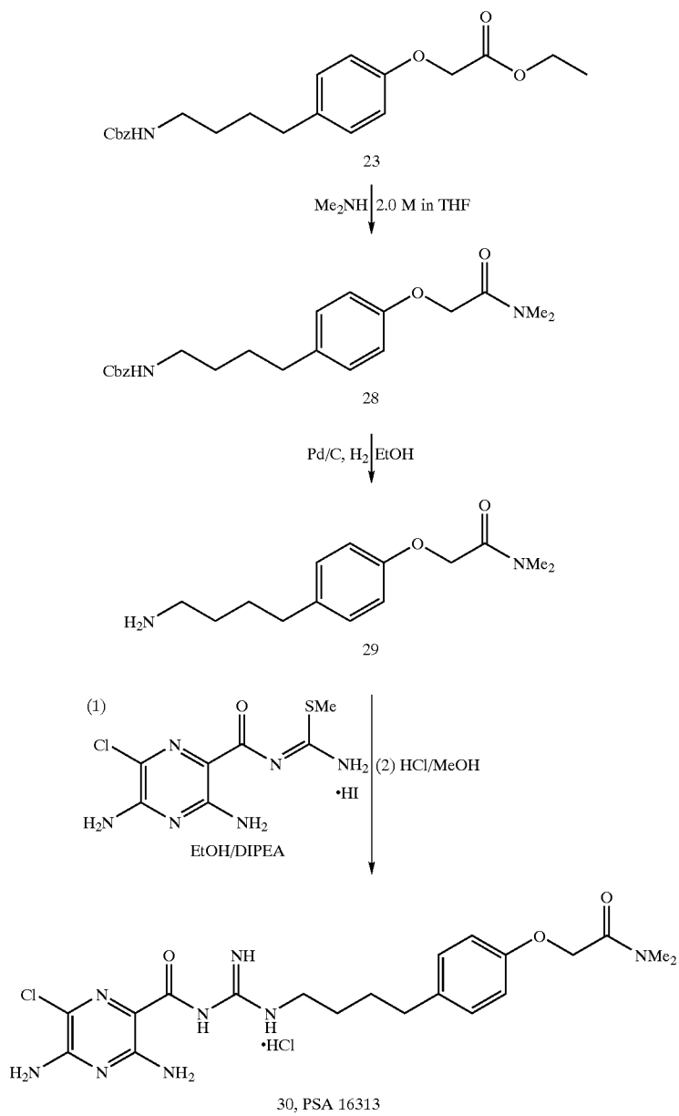
Scheme 7. Synthesis of PSA 16313
