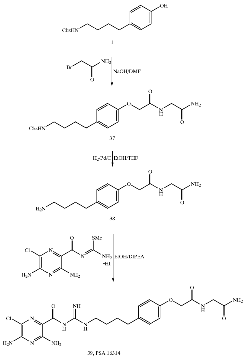
Scheme 9. Synthesis of PSA 16314
