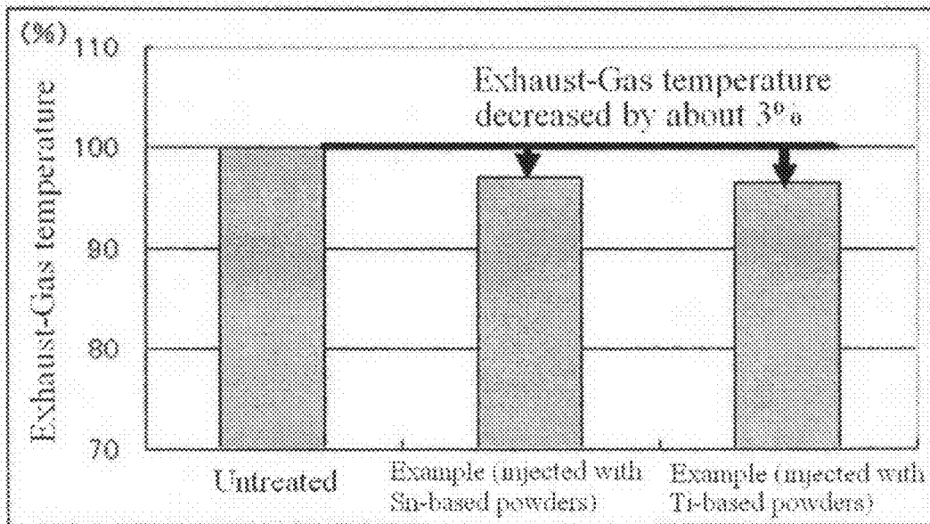
Graph for change in exhaust-gas temperature
