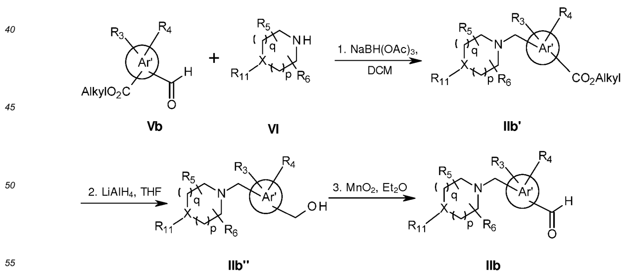
Scheme 5
