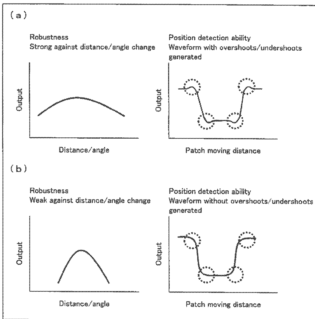
FIG. 21 PRIOR ART
