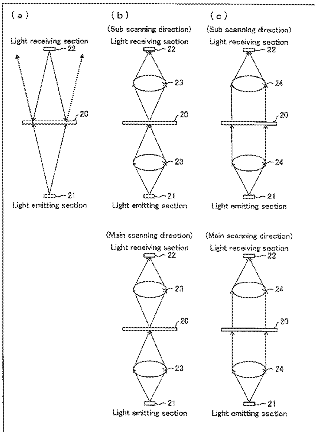
FIG. 5 PRIOR ART
