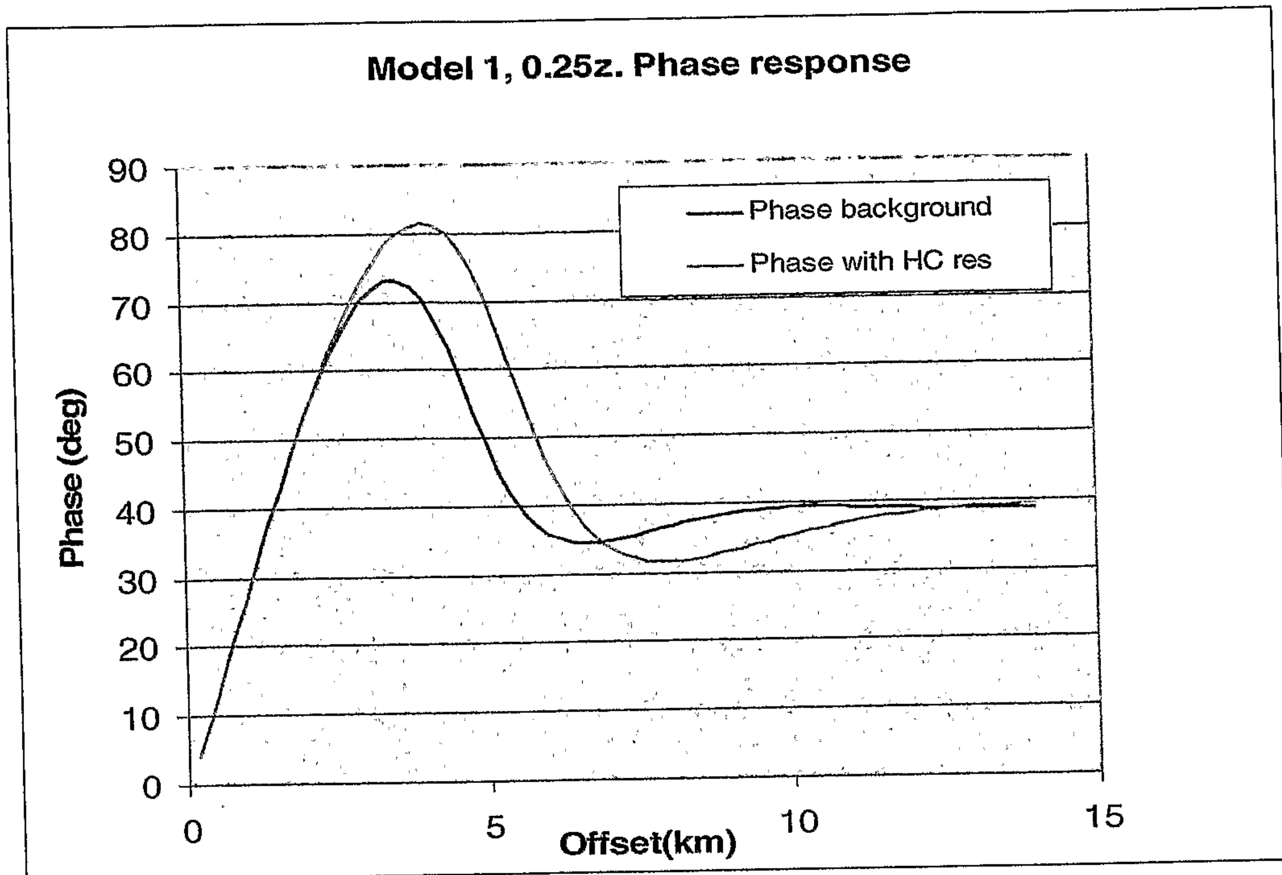
Fig. 3: Model 1, shallow water, 0.25 Hz. phase response
