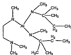
Compound No. 4
