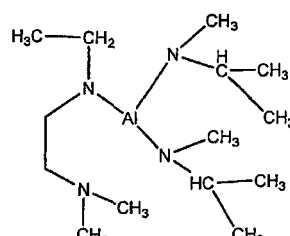
Compound No. 6
