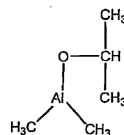
Comparative Compound 3
