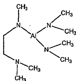
Comparative Compound 2
