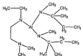
Compound No. 8
