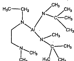
Compound No. 7
