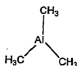
Comparative Compound 1
