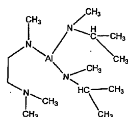
Compound No. 2
