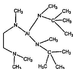
Compound No. 3
