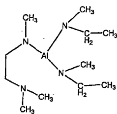
Compound No. 1
