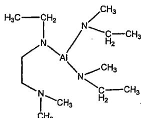
Compound No. 5
