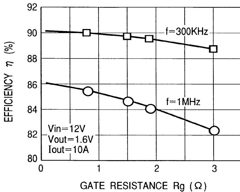
RELATION BETWEEN GATE RESISTANCE AND EFFICIENCY
