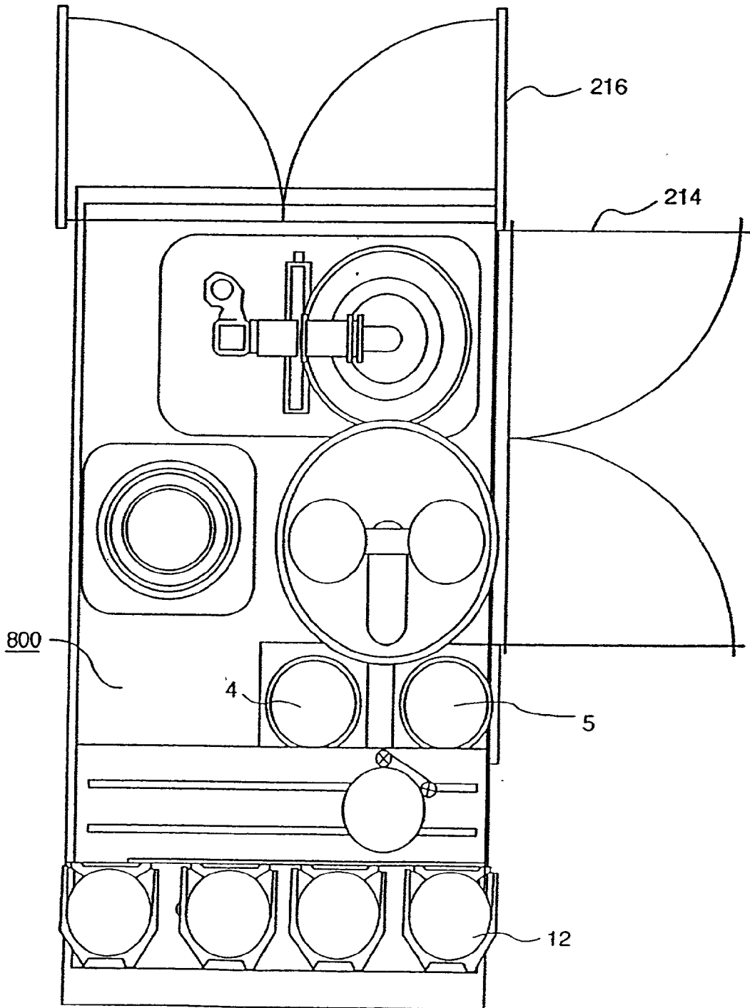
FIG. 9 PRIOR ART
