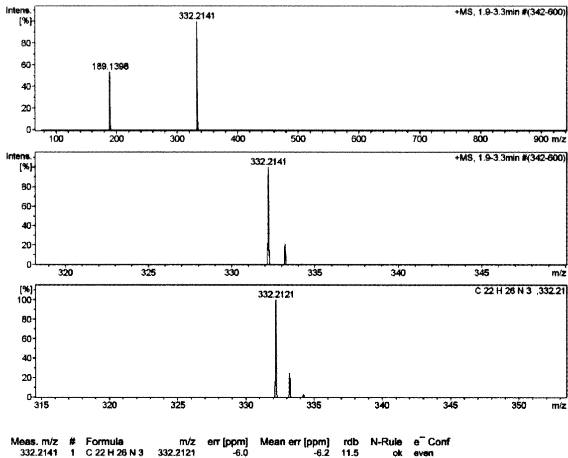
Figure 1(b) – Centhaquin citrate
