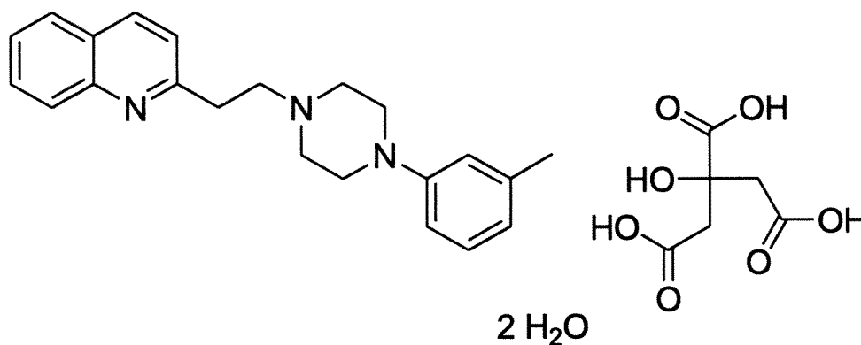
Structure of centhaquin citrate dihydrate
