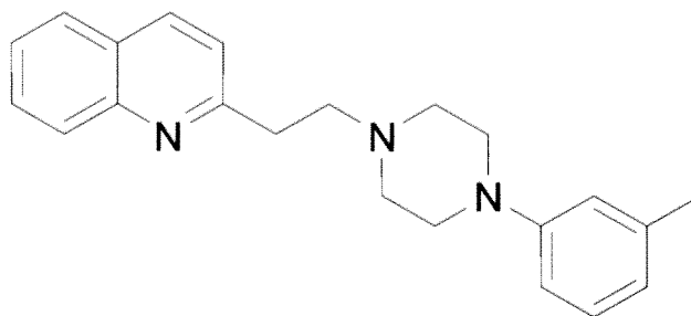
Structure of centhaquin (2-[2-(4-(3-methylphenyl)-1-piperazinyl) ethyl]-quinoline) (as free base)
