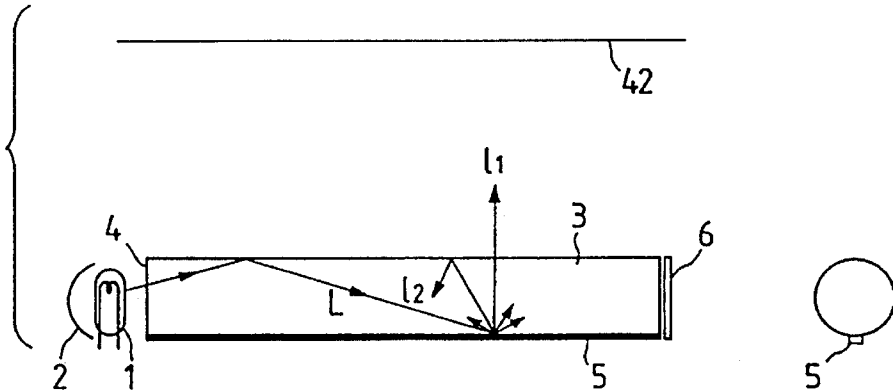
FIG. 5 PRIOR ART
