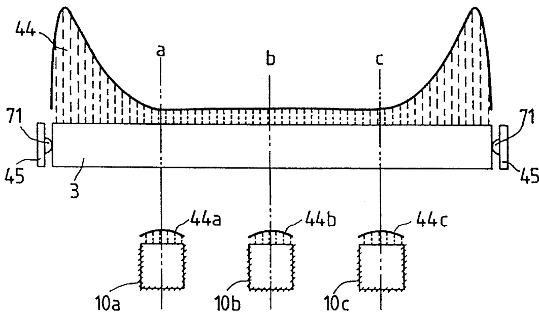
FIG. 9 PRIOR ART
