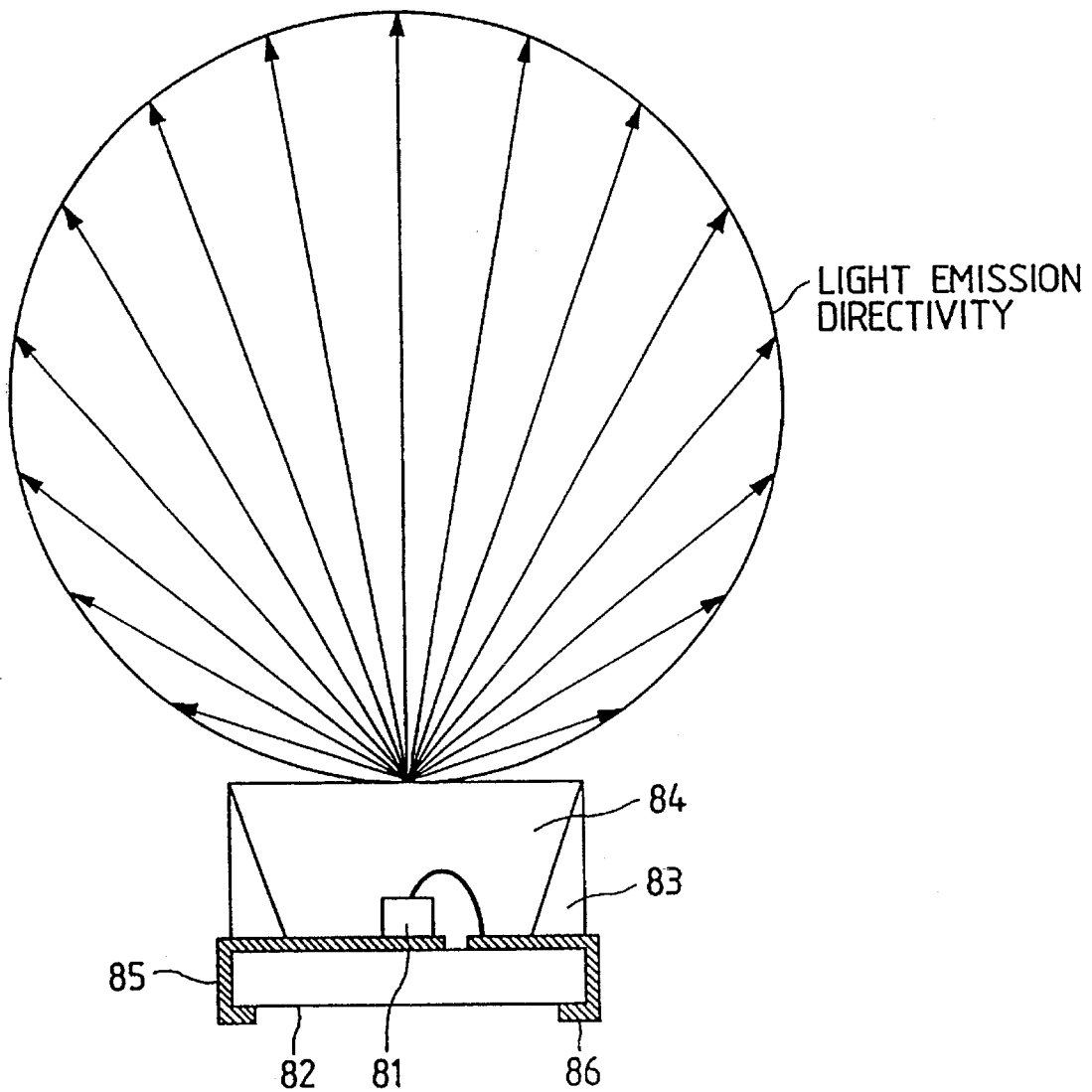
FIG. 7 PRIOR ART
