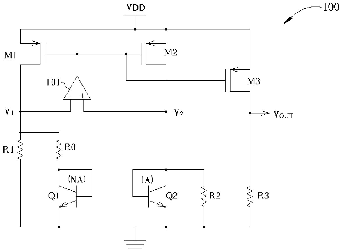
Fig. 1 Prior art
