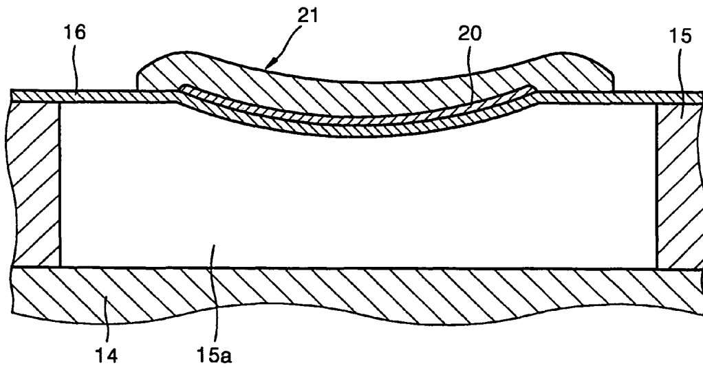
FIG. 4 (PRIOR ART)
