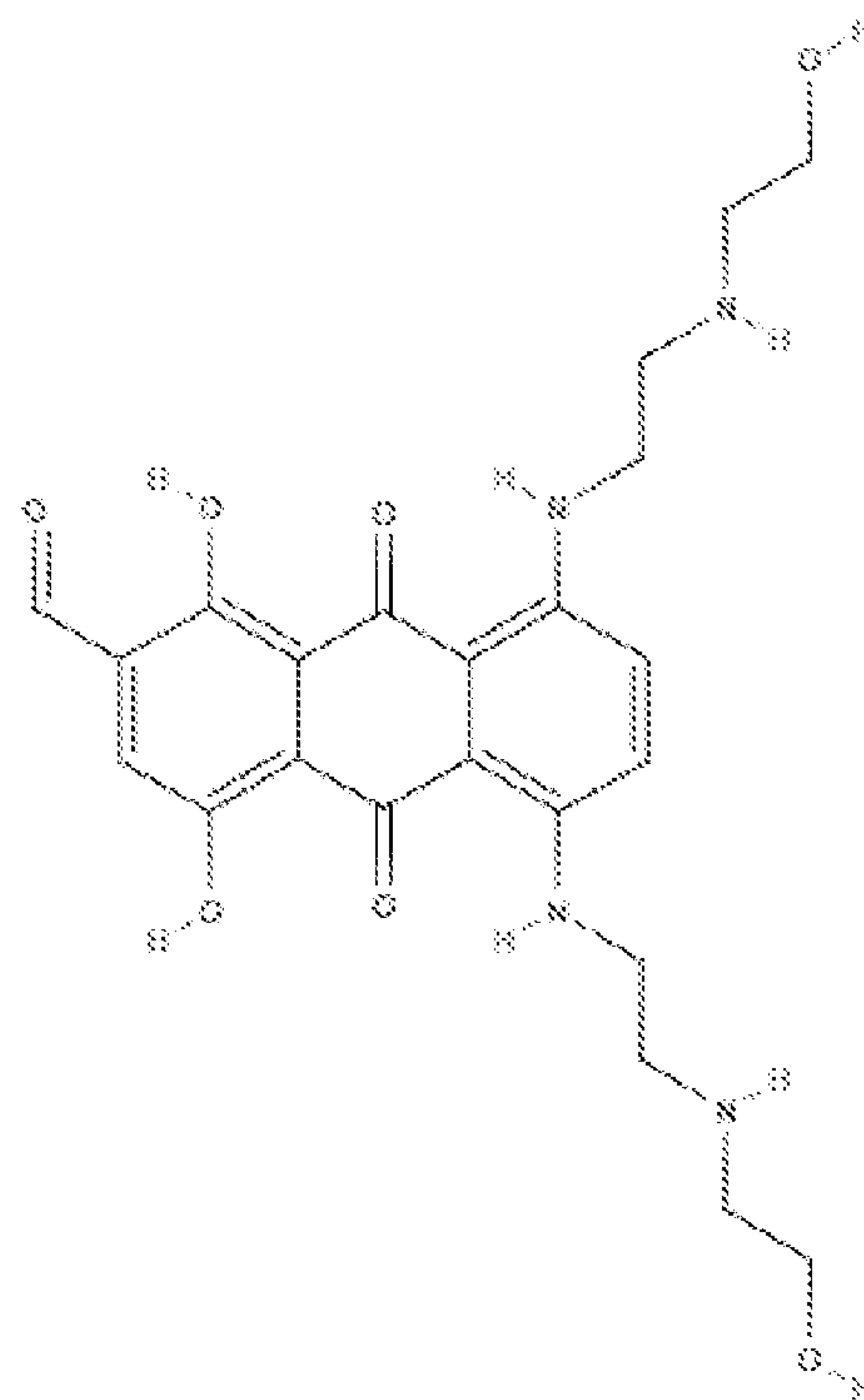
aldehyde XXXII
