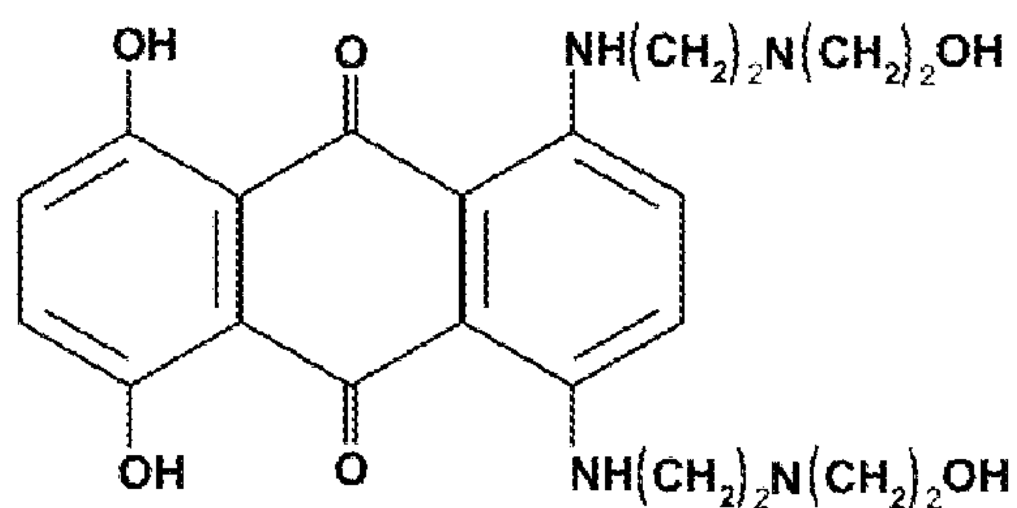
Mitoxantrone
