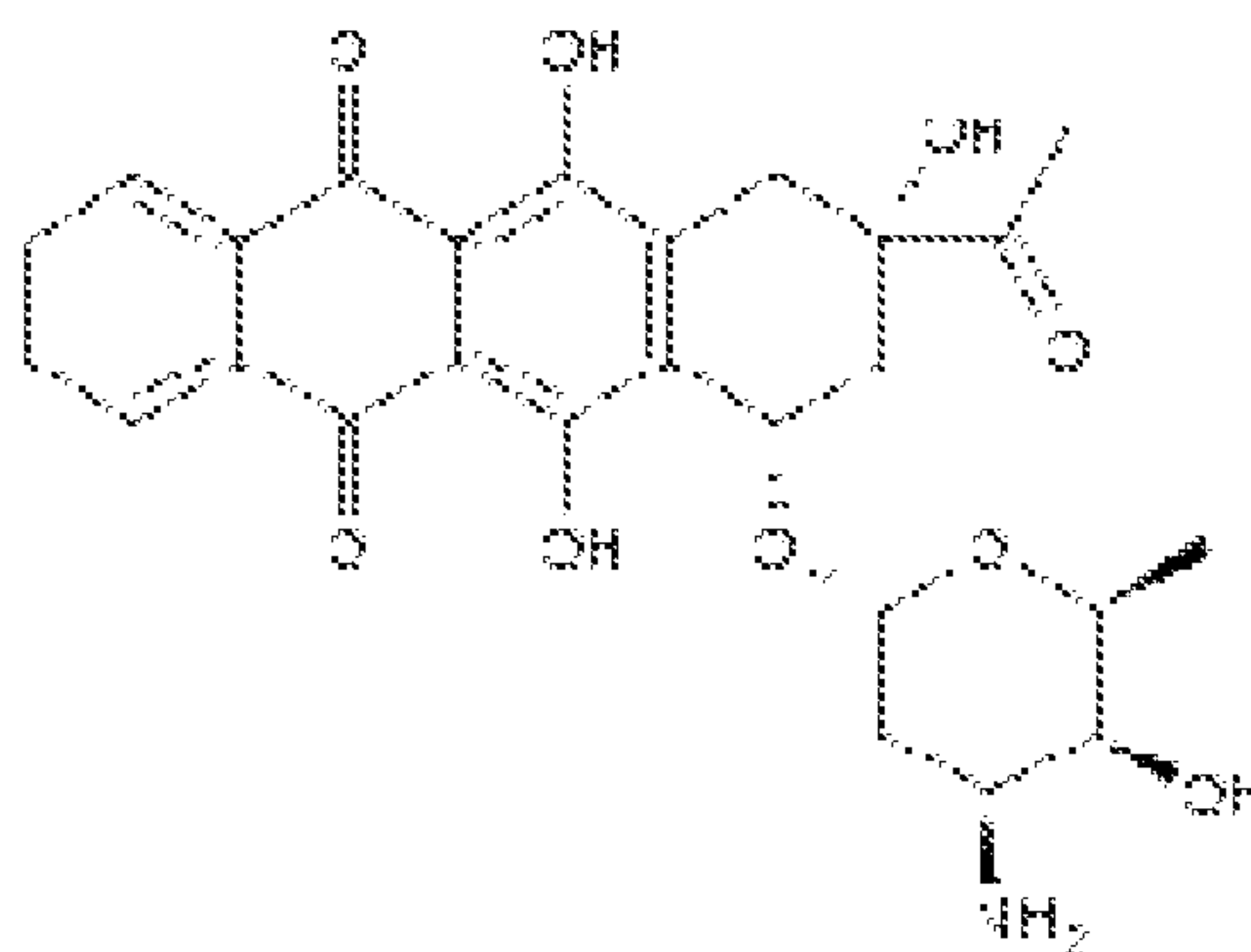
Idarubicin
