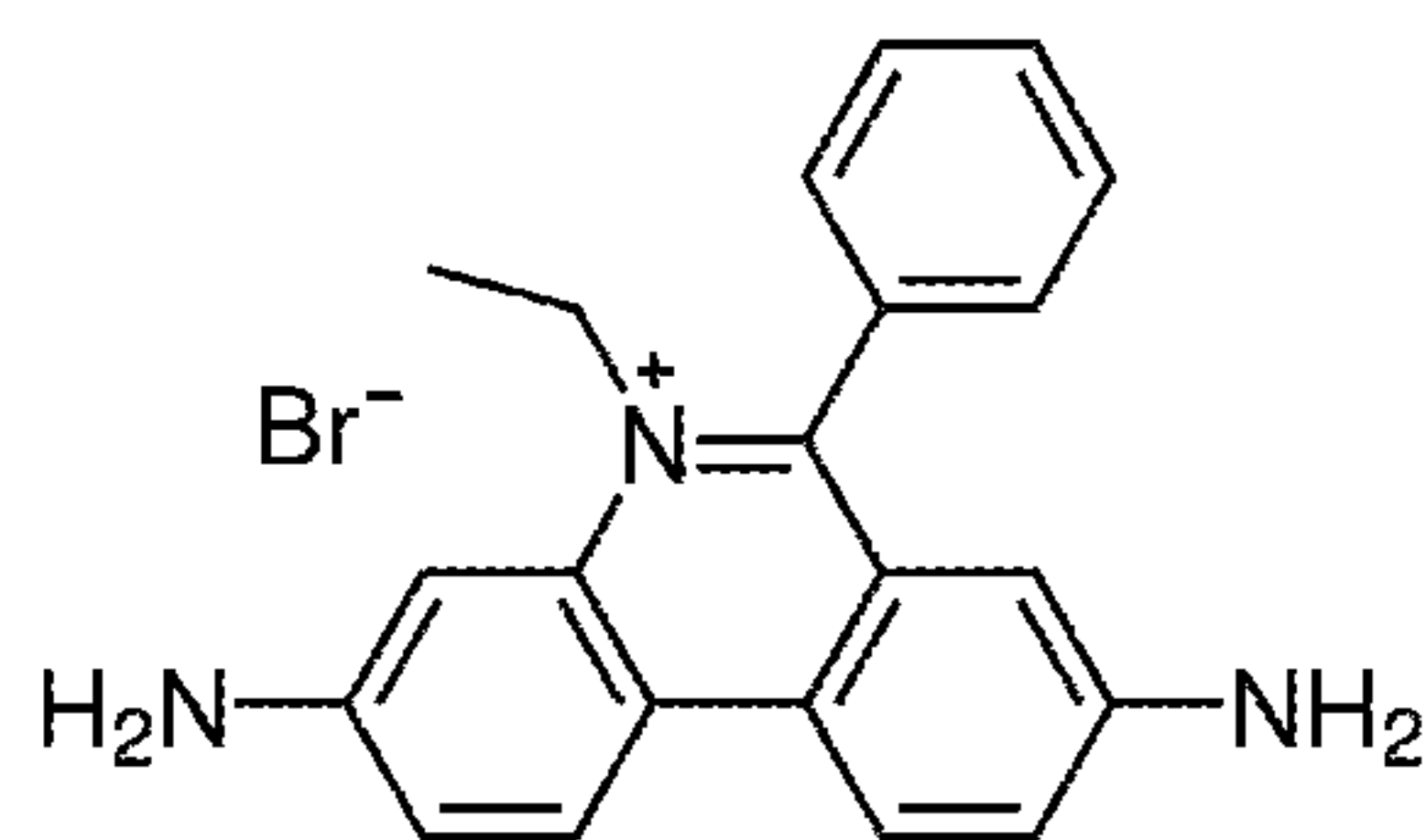
Ethidium bromide
