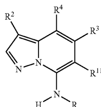
pyrazolopyridine
