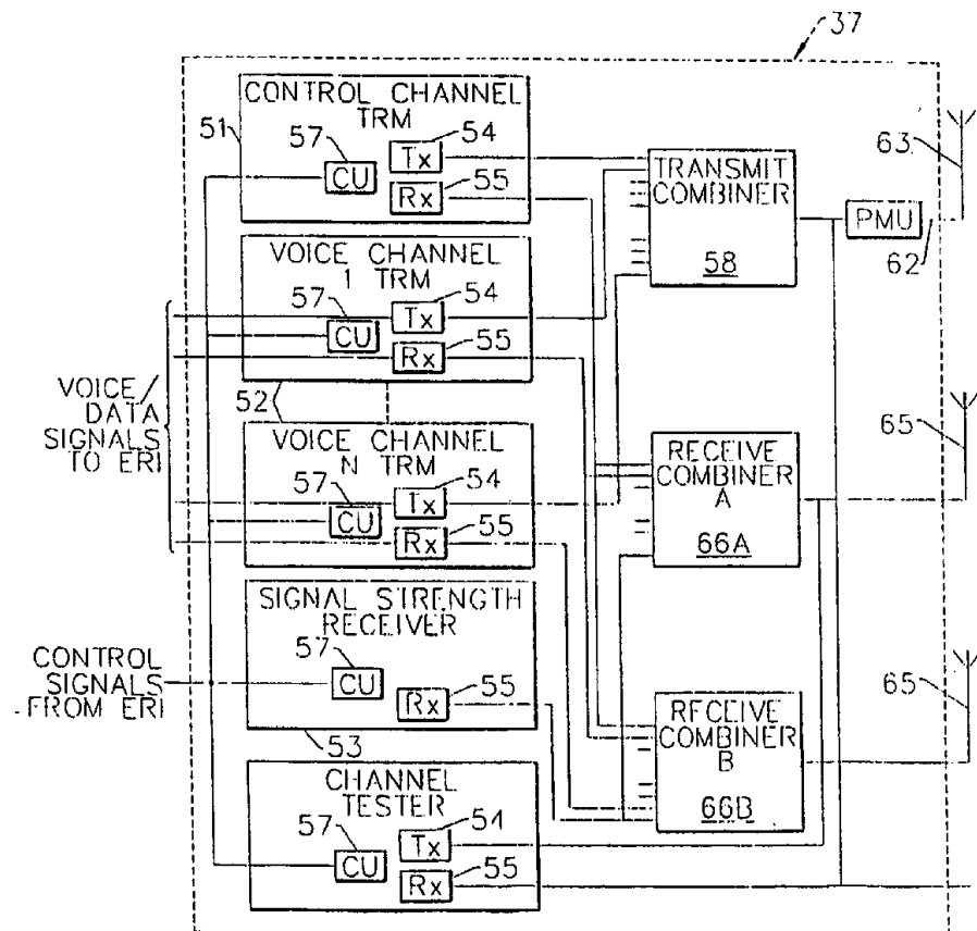
FIG. 3. (PRIOR ART)
