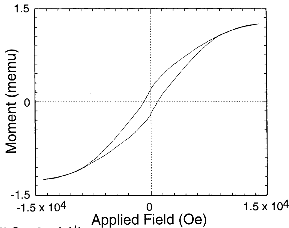
FIG. 25(d') Hard Axis Loop
