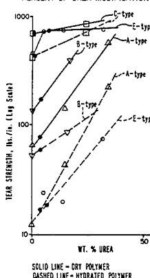
TEAR RESISTANCE vs. PERCENT OF UREA MODIFICATION
