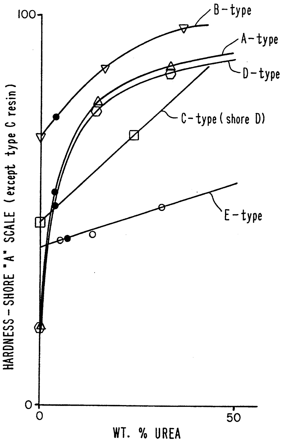
HARDNESS OF HYDRATED POLYMERS vs. PERCENT OF UREA MODIFICATION
