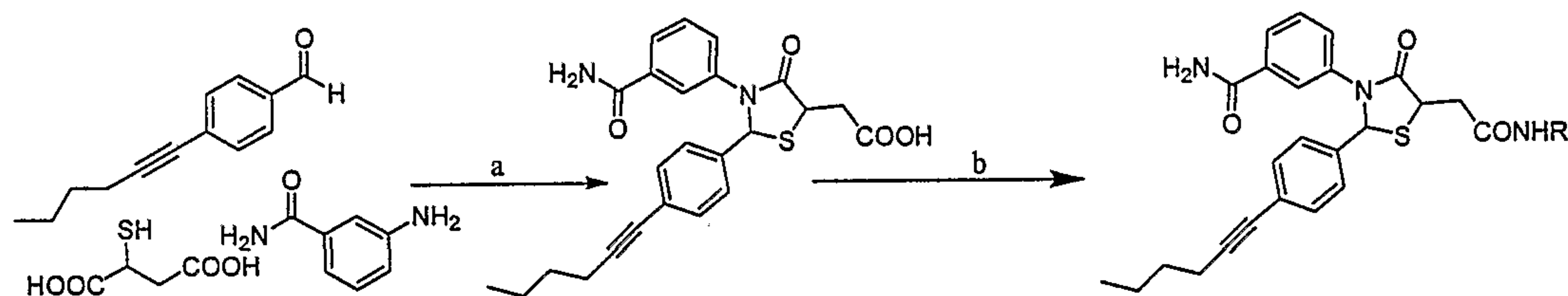
Scheme 1. For Examples 17-19
