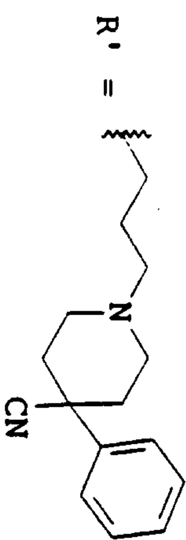
Scheme 14 (cont.). Preparation of example 28 (part-2)
