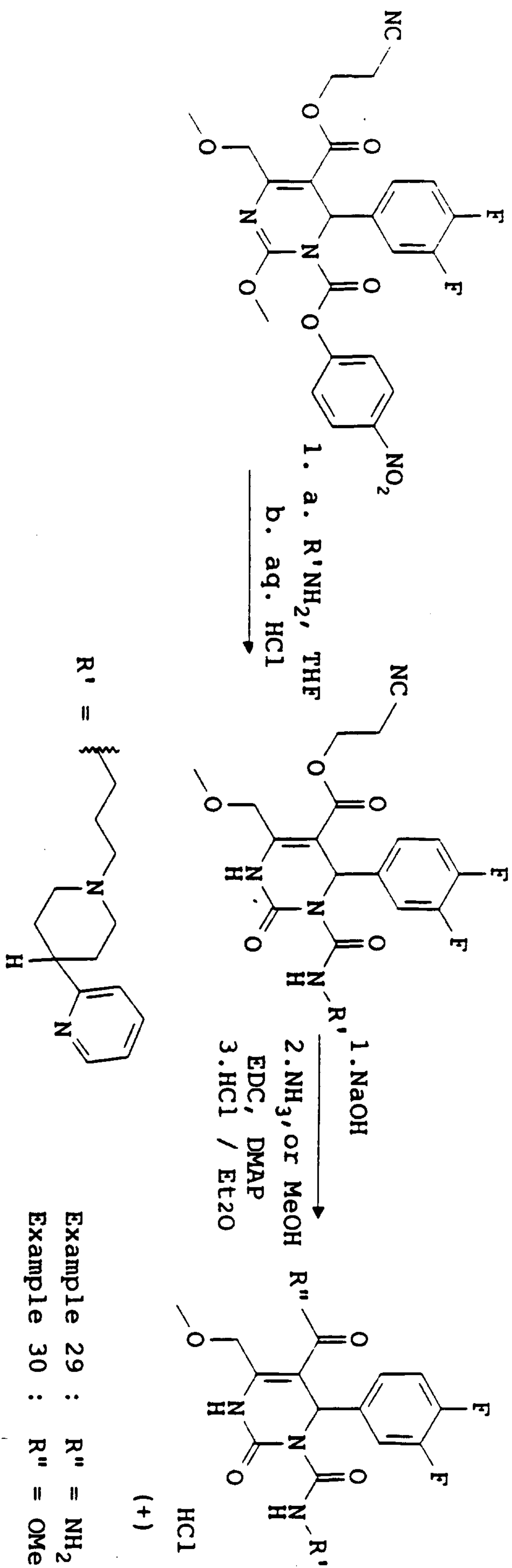
Scheme 15. Preparation of examples 29 and 30
