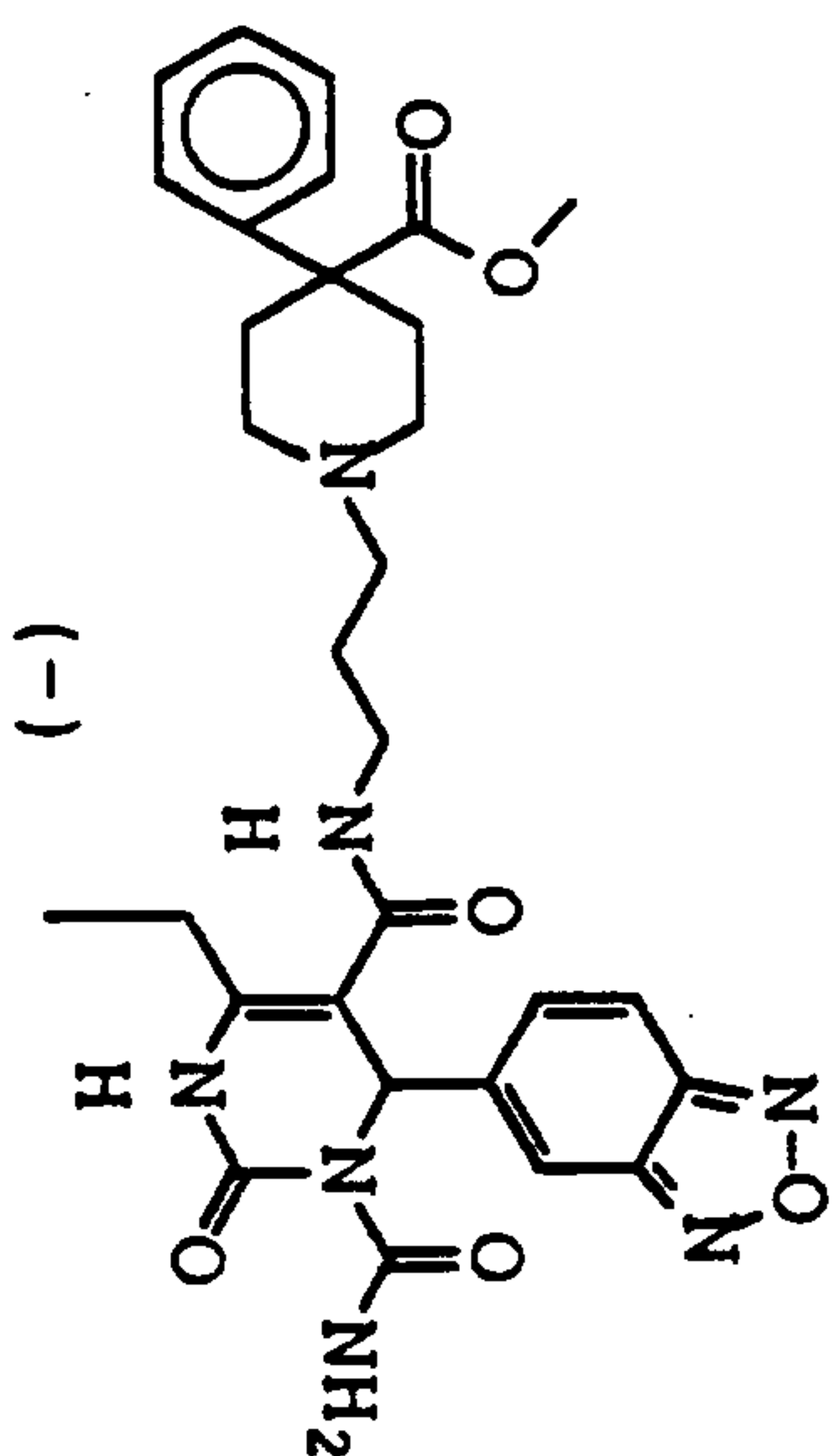
Scheme 13 (continued). Preparation of example 43 part-2
