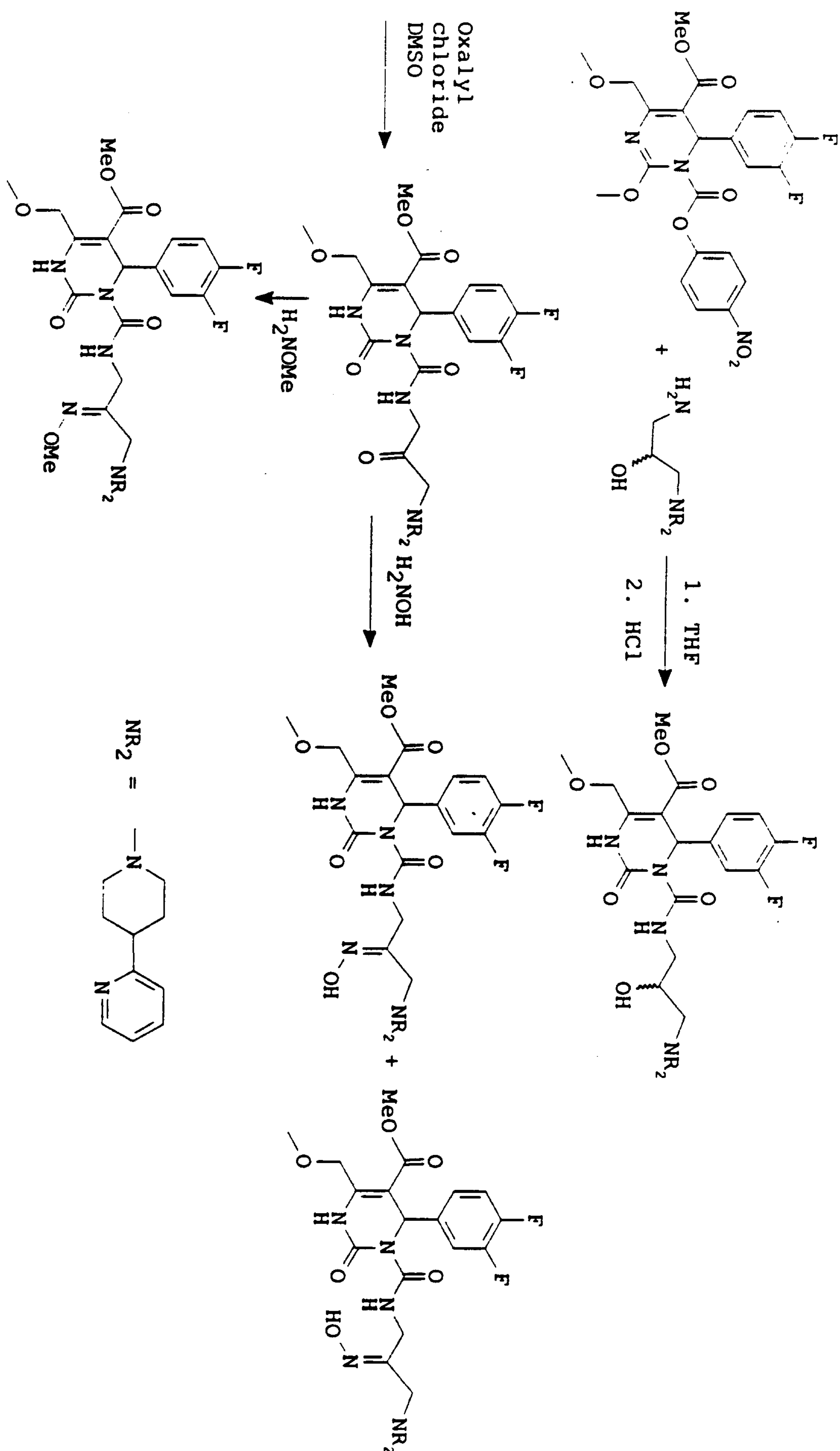
Scheme 17. Preparation of examples 31, 32, 33, and 34
