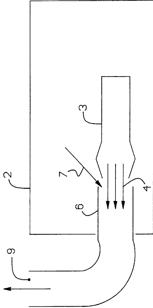
FIG 2 PRIOR ART
