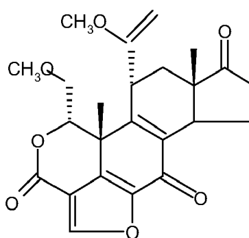
Wortmannin
