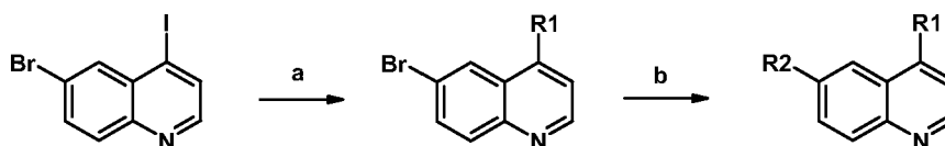
Scheme 16:
