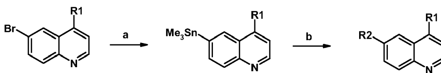
Scheme 6:
