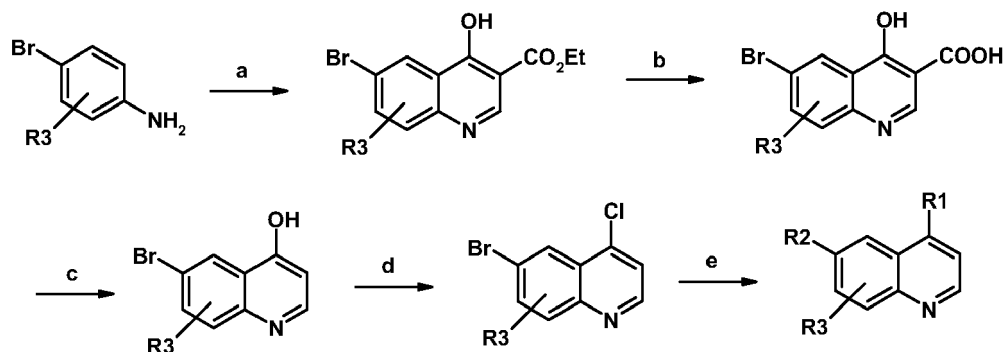
Scheme 7:
