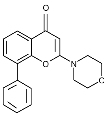
LY294002
