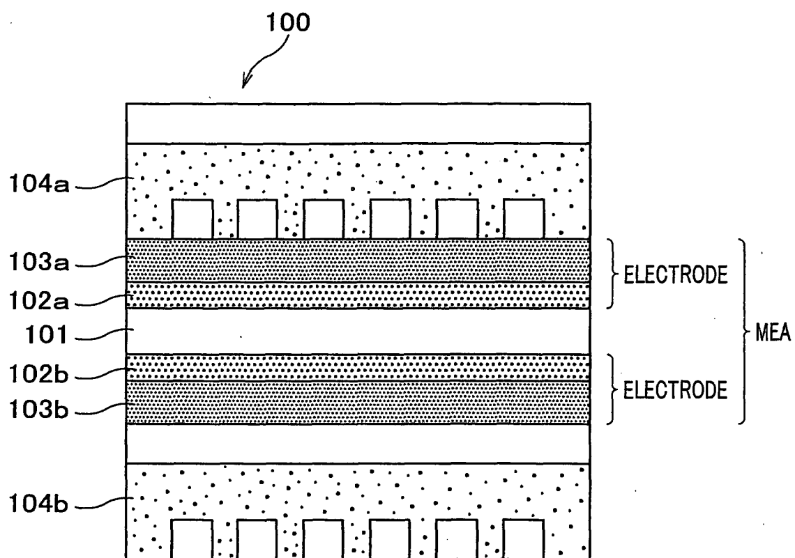
FIG. 8 PRIOR ART
