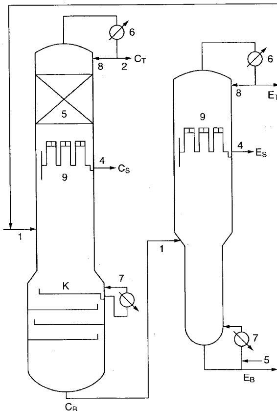
CONTINUOUS MULTI-STAGE DISTILLATION COLUMN C
