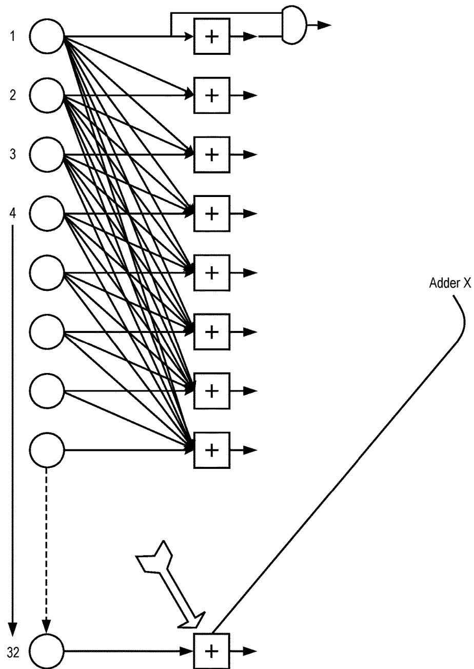
Parallel implementation of the adder tree
