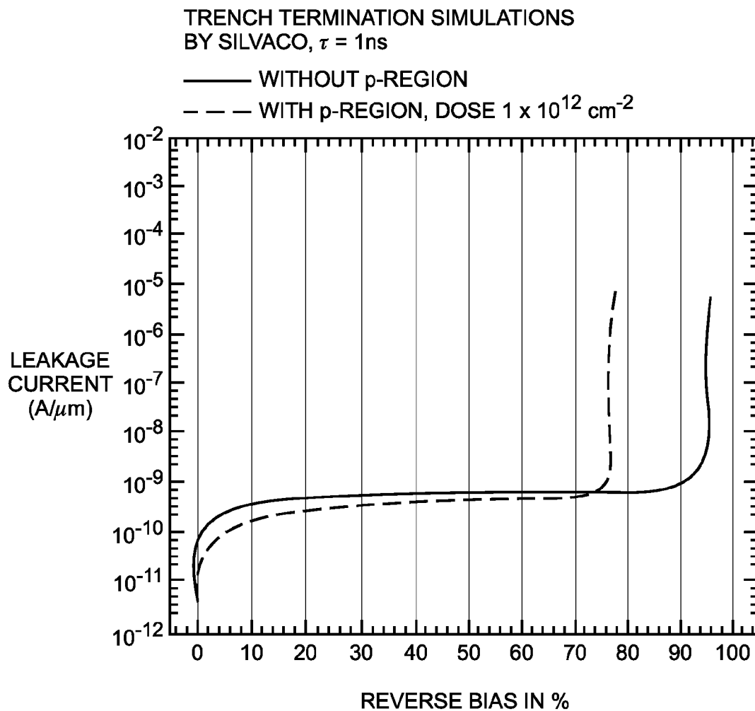
REVERSE CHARACTERISTICS
