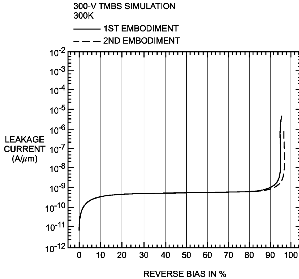
REVERSE CHARACTERISTICS
