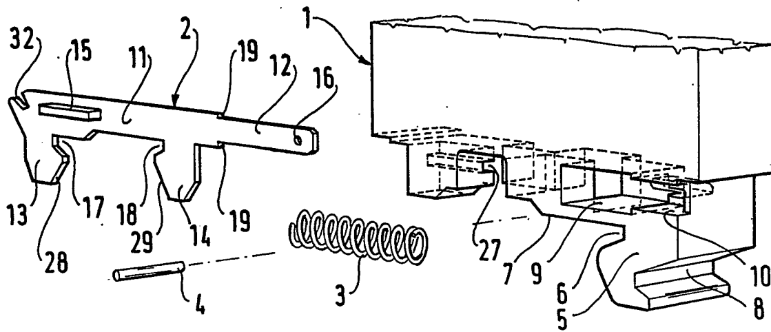
1/2 FIG.1
