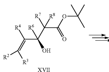
Scheme 3
