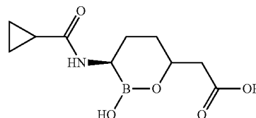
2-((3R)-3-(cyclopropanecarboxamido)-2-hydroxy-1,2-oxaborinan-6-yl)acetic acid 4
