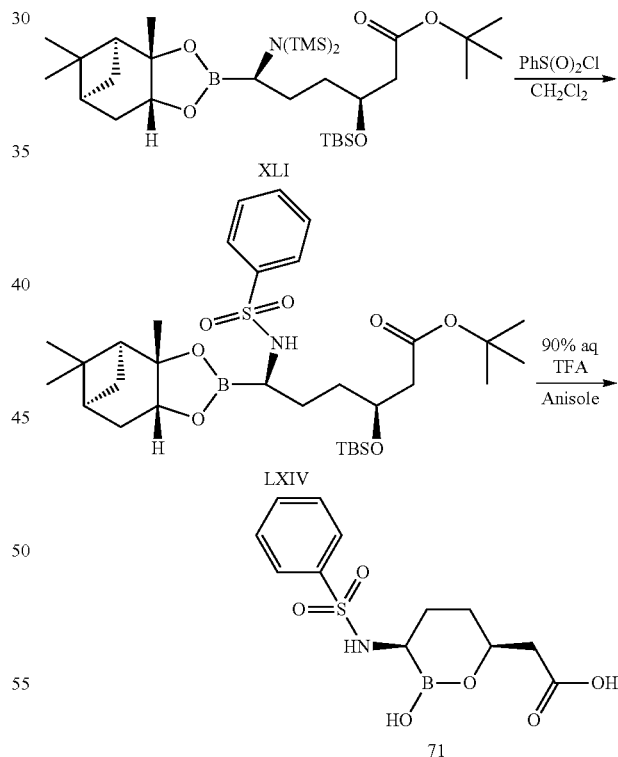
Scheme 17
