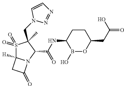
2-[(3R,6S)-2-hydroxy-3-[(2S,3S,5R)-3-methyl-4,4,7-trioxo-3-(1H-1,2,3-triazol-1-ylmethyl)-4 \lambda^6 -thia-1-azabicyclo[3.2.0]heptane-2-amido]-1,2-oxaborinan-6-yl]acetic acid 59
