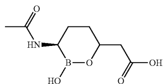
2-((3R)-3-acetamido-2-hydroxy-1,2-oxaborinan-6-yl)acetic acid 3
