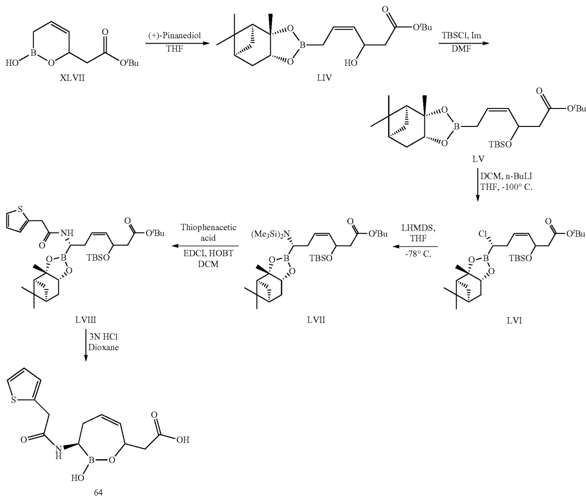
Scheme 12
