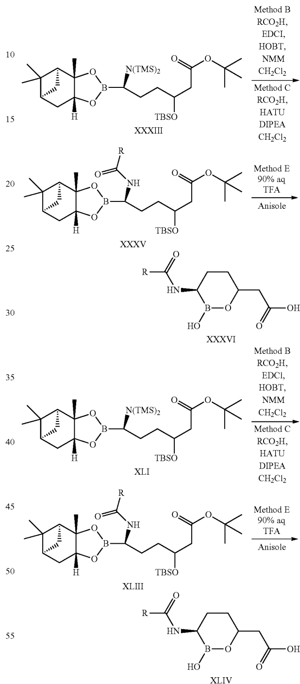
Scheme 9
