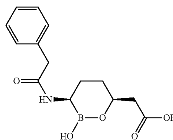
2-((3R,6S)-2-hydroxy-3-(2-phenylacetamido)-1,2-oxaborinan-6-yl)acetic acid 6
