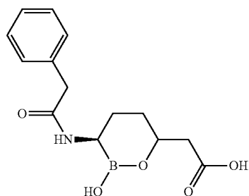
2-((3R)-2-hydroxy-3-(2-phenylacetamido)-1,2-oxaborinan-6-yl)acetic acid 2
