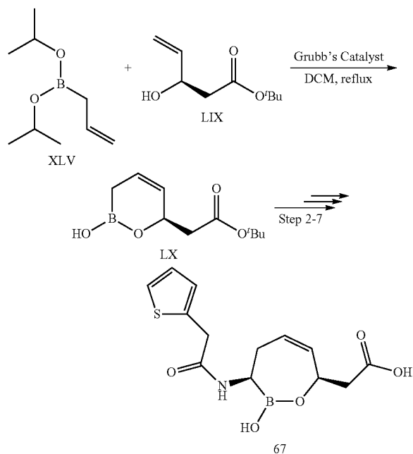
Scheme 14
