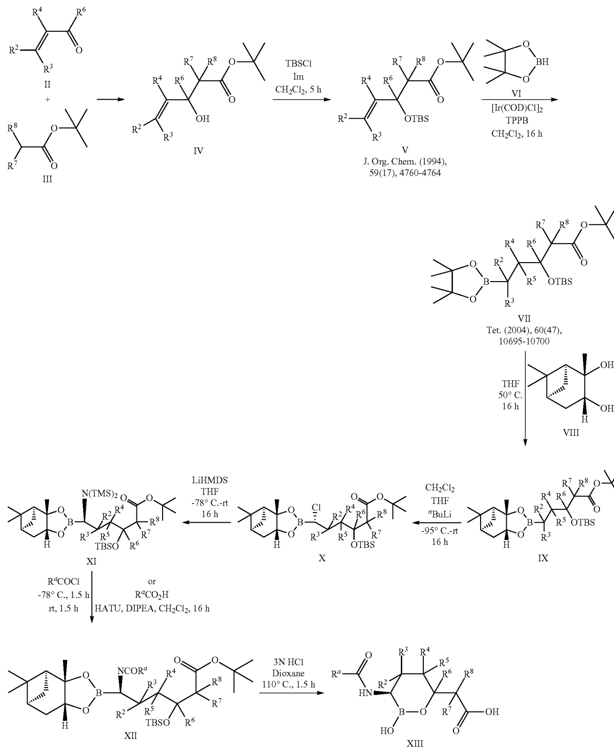
Scheme 1
