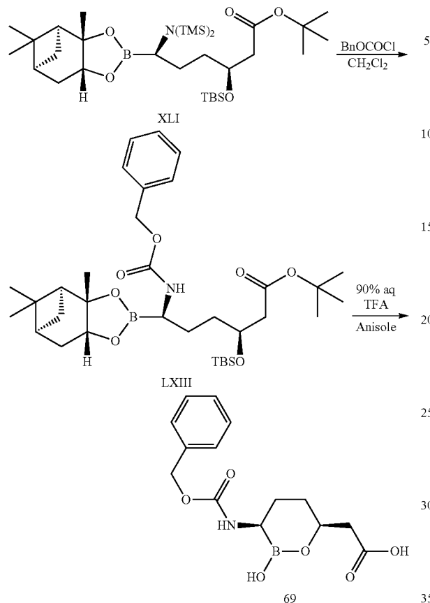
Scheme 16
