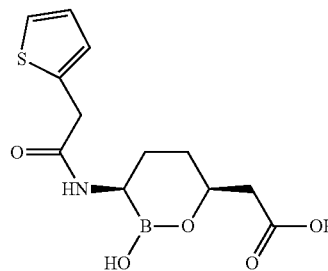
2-((3R,6S)-2-hydroxy-3-(2-(thiophen-2-yl)acetamido)-1,2-oxaborinan-6-yl)acetic acid 5
