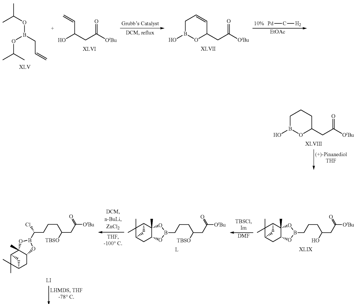
Scheme 11
