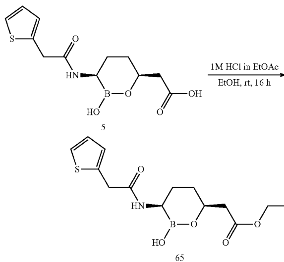
Scheme 13
