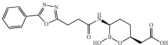
2-[(3R,6S)-2-hydroxy-3-(3-(5-phenyl-1,3,4-oxadiazol-2-yl)propanamido)-1,2-oxaborinan-6-yl]acetic acid 60
