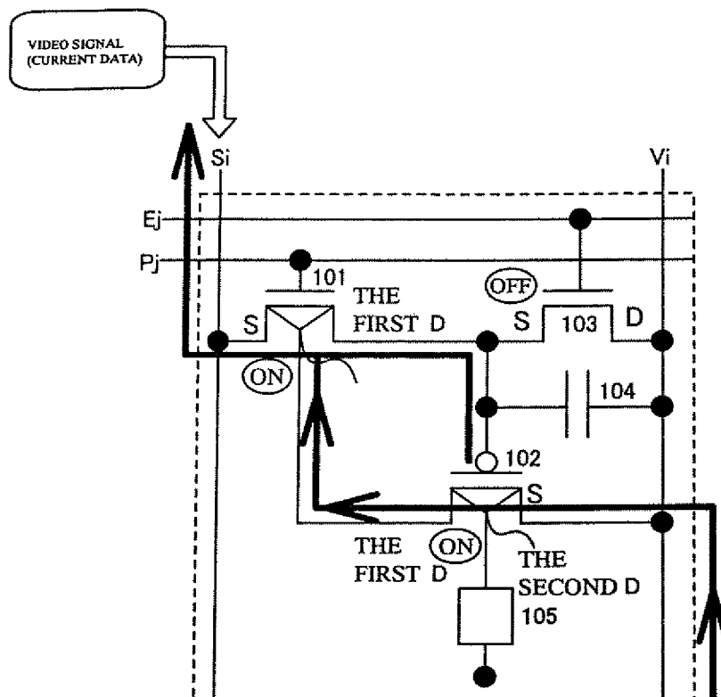
Fig.4A WRITING PERIOD T_a
