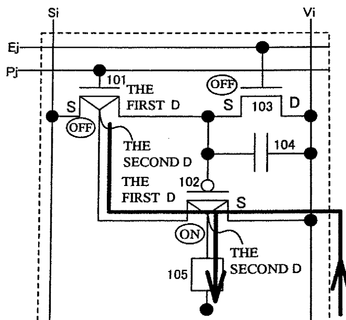
Fig.4B DISPLAYING PERIOD T_d
