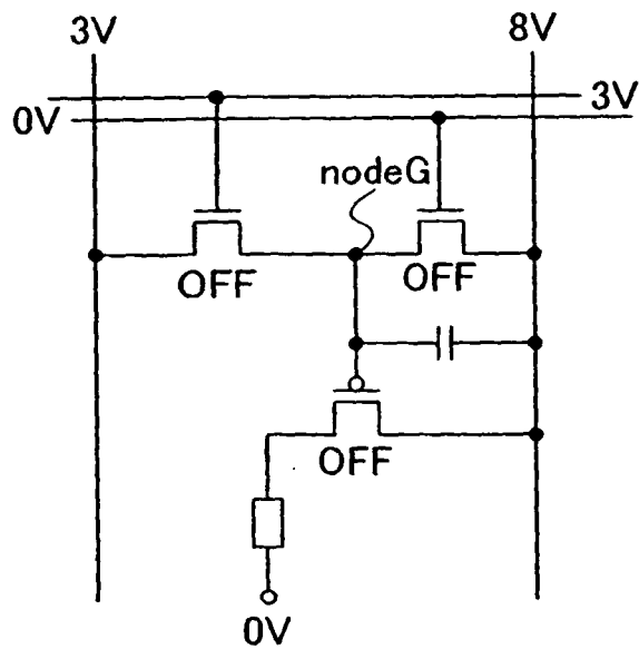
FIG. 4B sustain period (non-light emitting signal input period)
