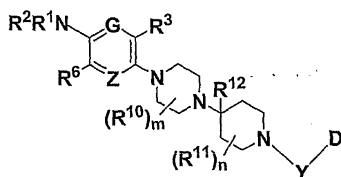
Formula 1
