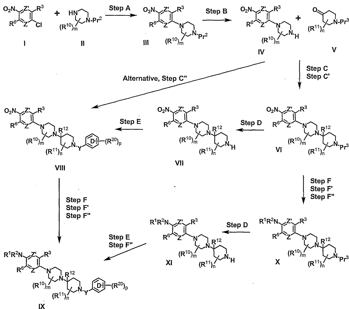
Scheme 1
