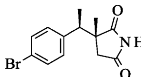
Minor diastereomer
