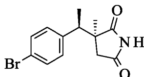
Major diastereomer
