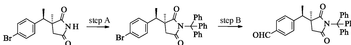
Scheme 2
