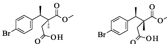
Major diastereomer
