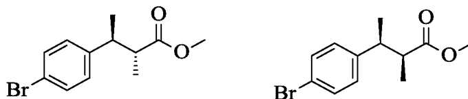
Major diastereomer
