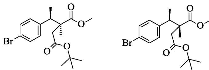
Major diastereomer
