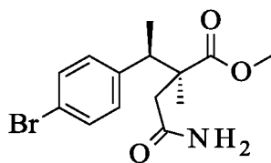
Major diastereomer
