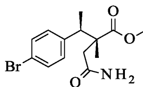
Minor diastereomer
