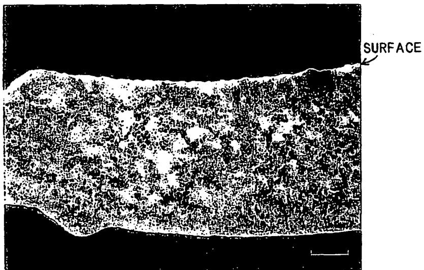
CONVENTIONAL PRODUCT SECTION \times 10
