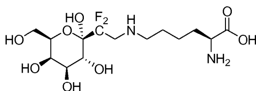
Compound 4,
