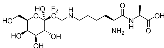
Compound 3,
