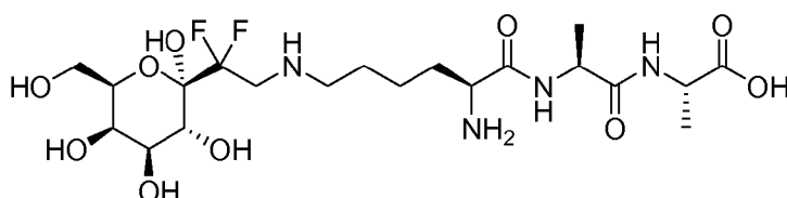
Compound 1,
