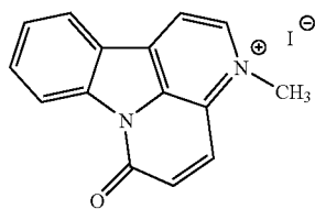
\text{C}_{15}\text{H}_{11}\text{IN}_2\text{O} - MW 362
