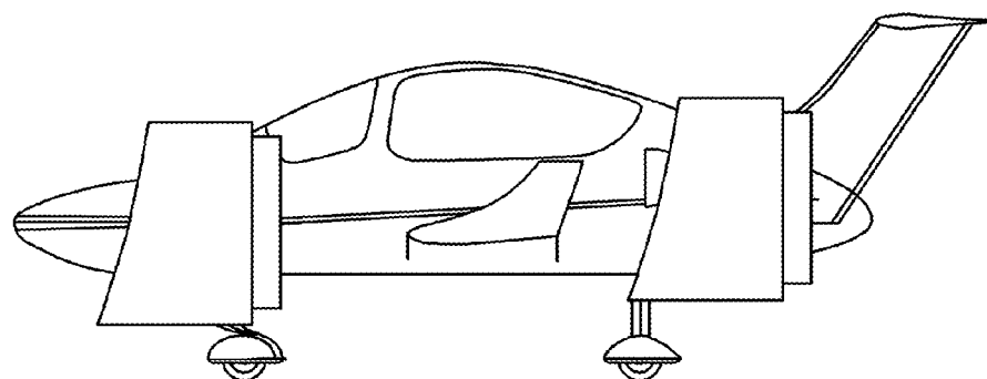
DUCT POSITION-FORWARD FLIGHT WITH FORWARD THRUST
