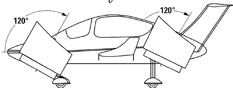
DUCT POSITION-BRAKING POSITION WITH REVERSE THRUST
