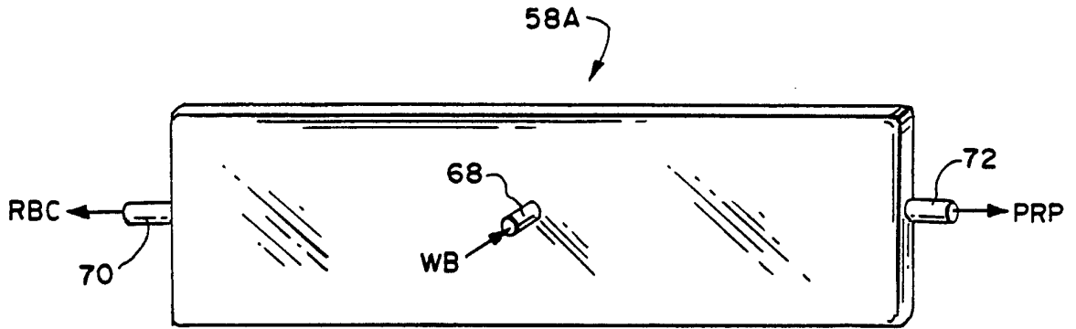
FIG. 14 PRIOR ART
