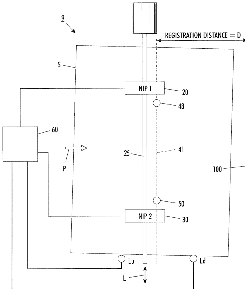
FIG. 5 PRIOR ART
