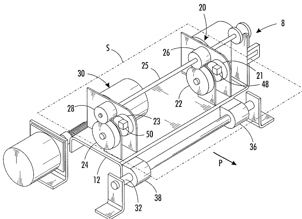
FIG. 4 PRIOR ART
